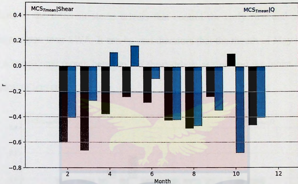
Figure 40: Mean MCS temperatures with wind shear (black bars) and 925 hPa specific humidity (blue bars) over Coastal sub-division of SWA.
