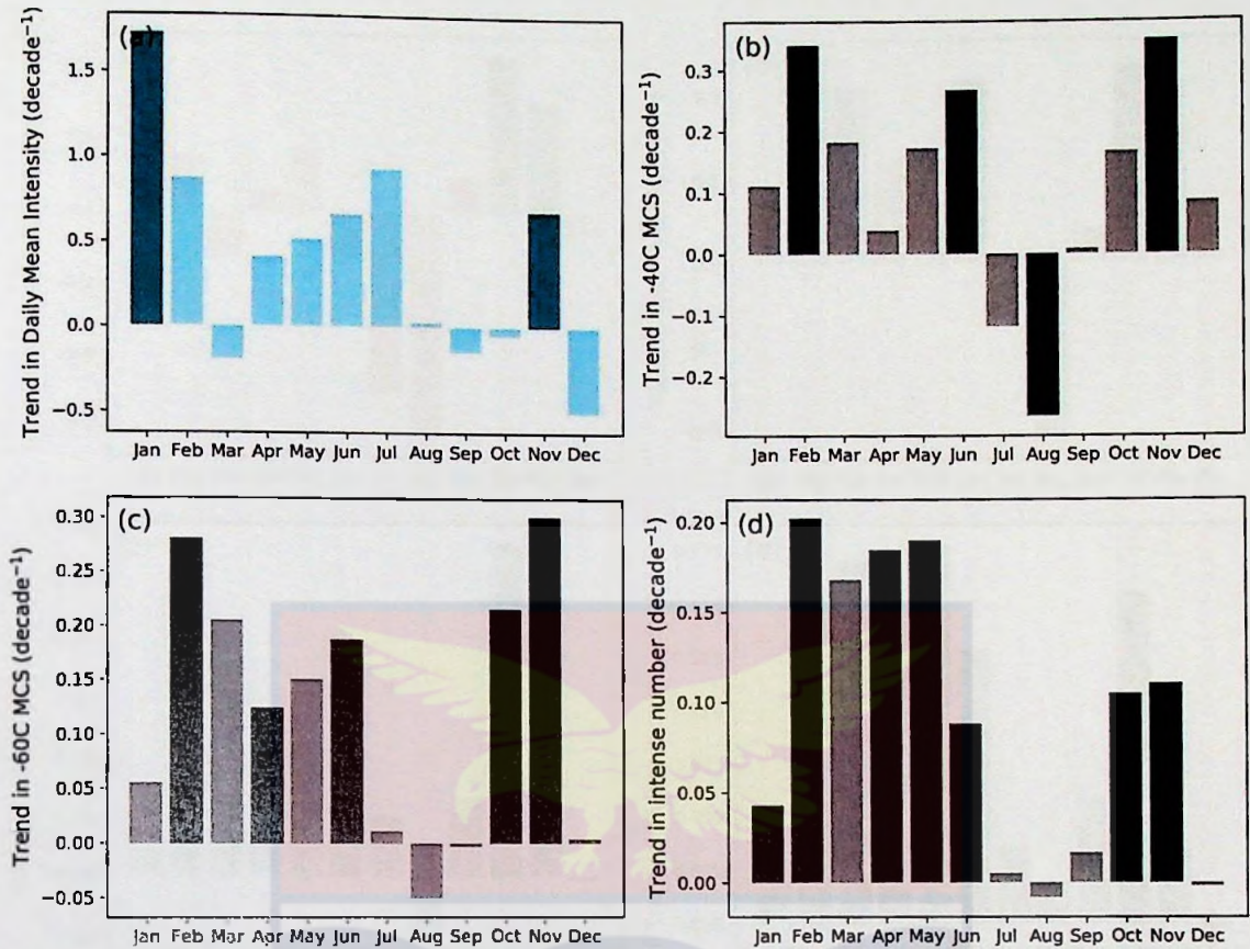
Figure 46: Same as figure 44, but for mean intensity of rainfall
