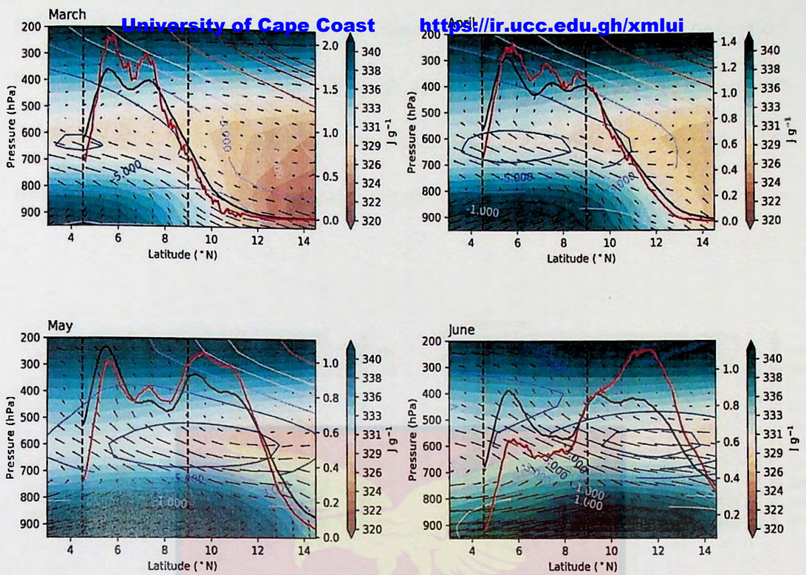
Figure 51: Monthly average 1200 UTC cross-sections between 10°W to 10°E of the moist static energy (shading, J g^{-1} ), meridional wind vectors ( m s^{-1} , w-component was multiplied by 10 for better visibility) and average frequency of MCSs (black line) and intense MCSs (red line) at 1800 UTC for March, April, May and June.
