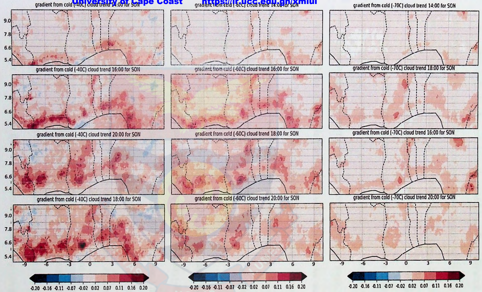
Figure 28: Same as figure 27, but for SON.
