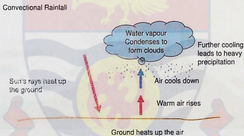
Figure. 5: Diagram showing the formation of convectional rainfall.
