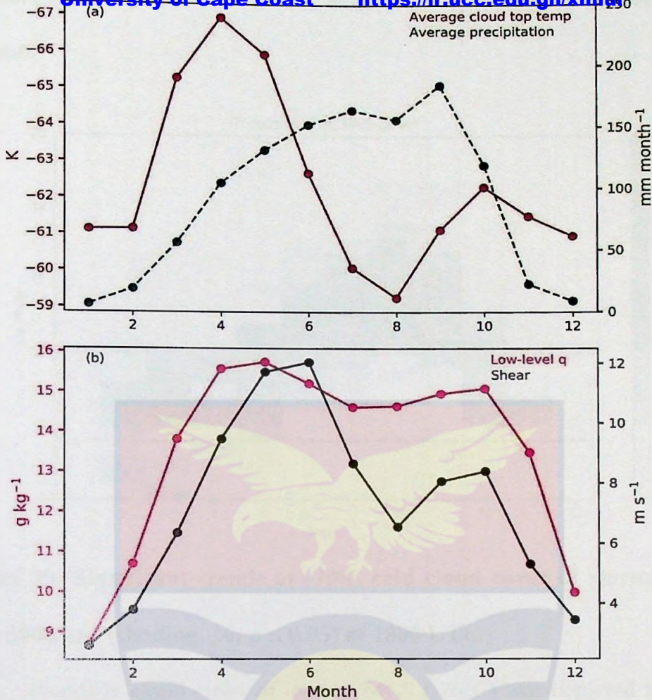
Figure 38: Same as figure 37, but for the Inland sub-division of SWA.
