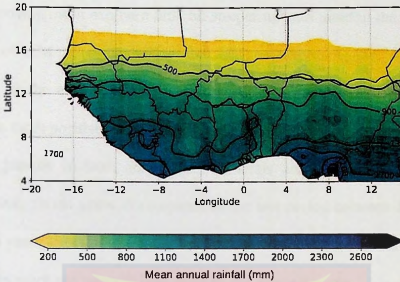
Figure 20: Average annual rainfall calculated over the period 1970 - 2014
