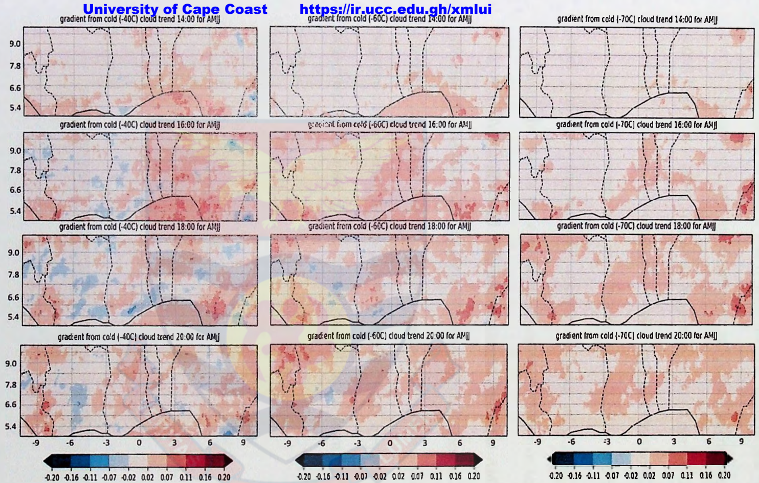
Figure 27: Significant trends ( P < 0.05 ) in MCS cloud cover at 1400,1600, 1800 and 2000 UTC using temperature thresholds of -40^{\circ}\text{C} , -60^{\circ}\text{C} and -70^{\circ}\text{C} for AMJJ
