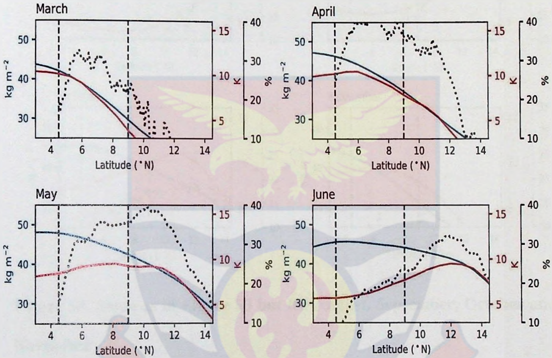
Figure 53: Plots of total column water vapour (blue, \text{kg m}^{-2} , \Delta\theta_e (red, K) and the contribution of intense MCSs to the total of MCSs (dotted, %).
