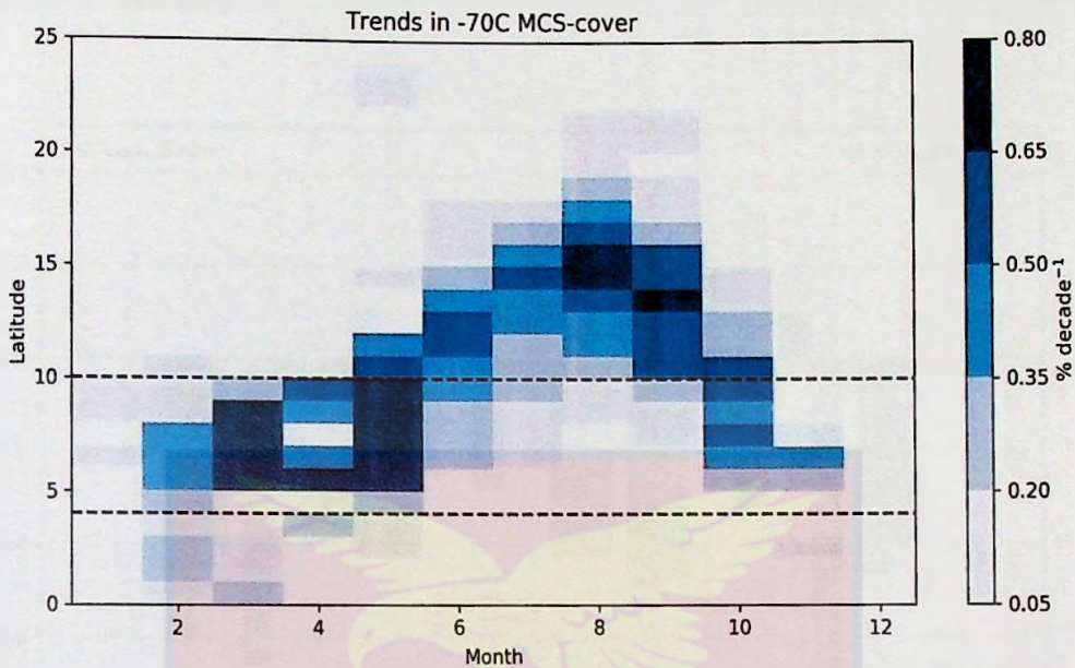
Figure 39: Significant trends at -70°C cold cloud cover of storms larger than 5000 km 2 (shading, %, p \leq 0.05 ) at 1800 UTC
