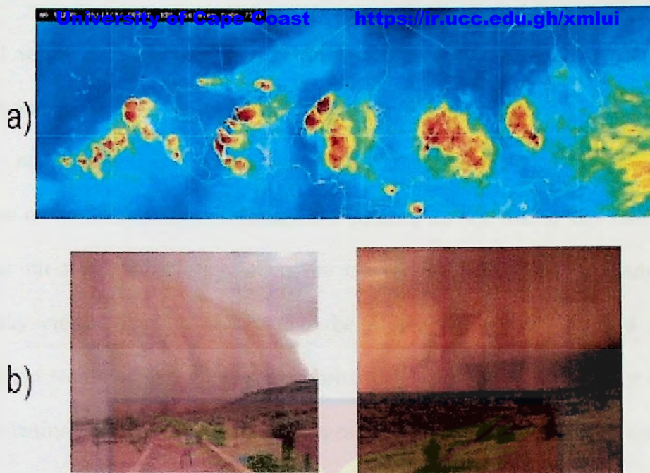
Figure 15. Mesoscale Convective Systems in West Africa. (a) Seen by infrared satellite - weather image (b) Seen from the ground photo (Panthou, 2013)
