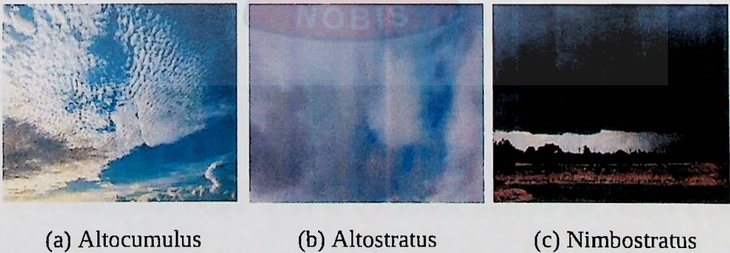
Figure 9 Mid-level clouds (Source: metoffice uk, 2019)
