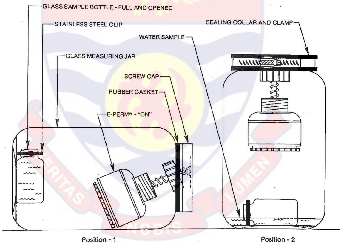
Figure 3.6: E-PERM ® system (radon-in-water measurement)
