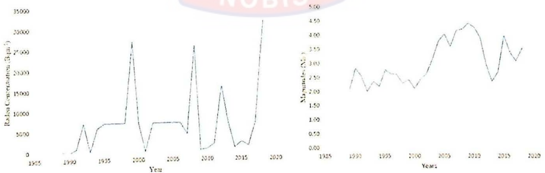
Figure 4.16: Pearson’s Correlation Plot (1836-2018)
