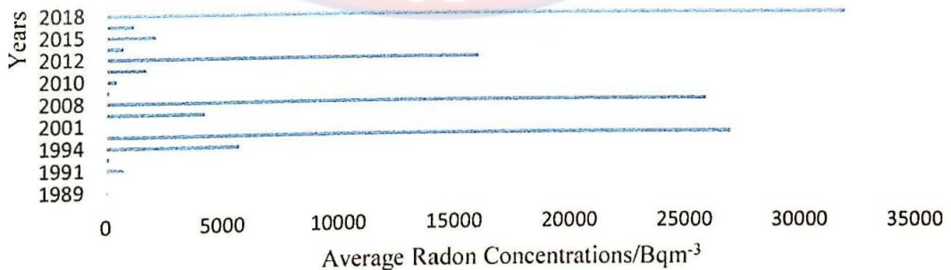
Figure 4.14: Plot of Yearly Average Radon Concentrations
