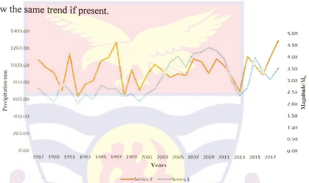
Figure 4.12: Plot of Precipitation Against Average Seismicity
