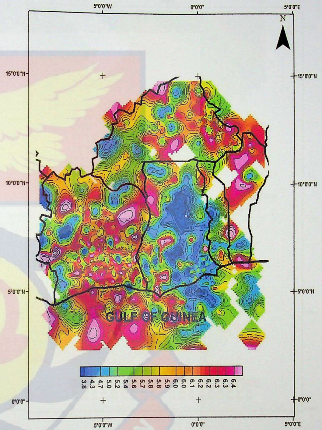
Figure 4.10: Isoseismal Map of Ghana and Its Immediate Neighbours
