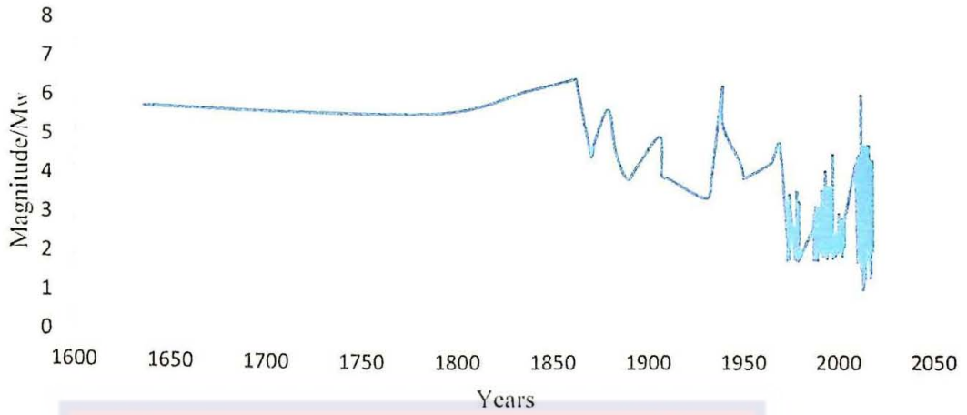
Figure 4.1: Plot of the Magnitude of the Seismic Events from 1615-2018
