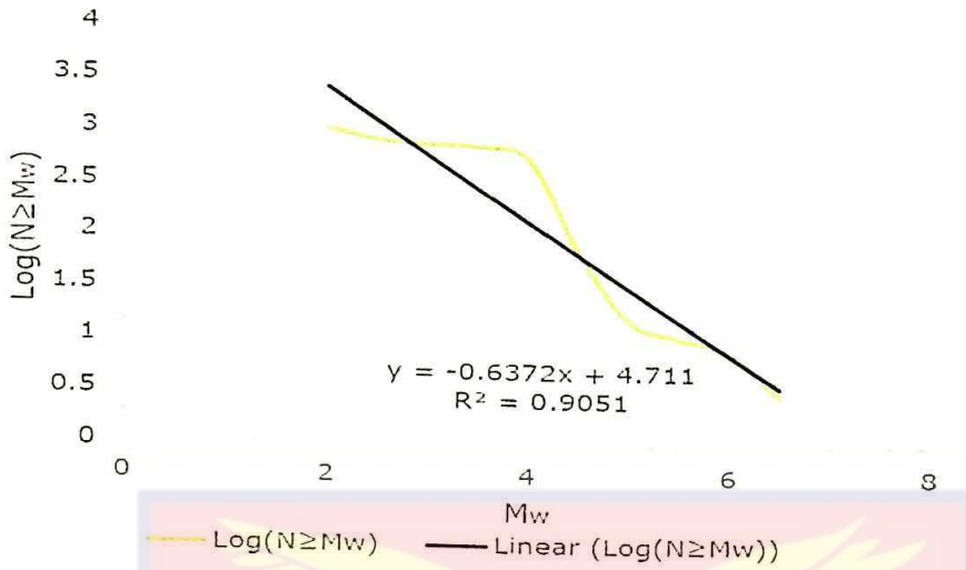
Figure 4.4: Gutenberg-Richter Model Plot (1615-2015)
