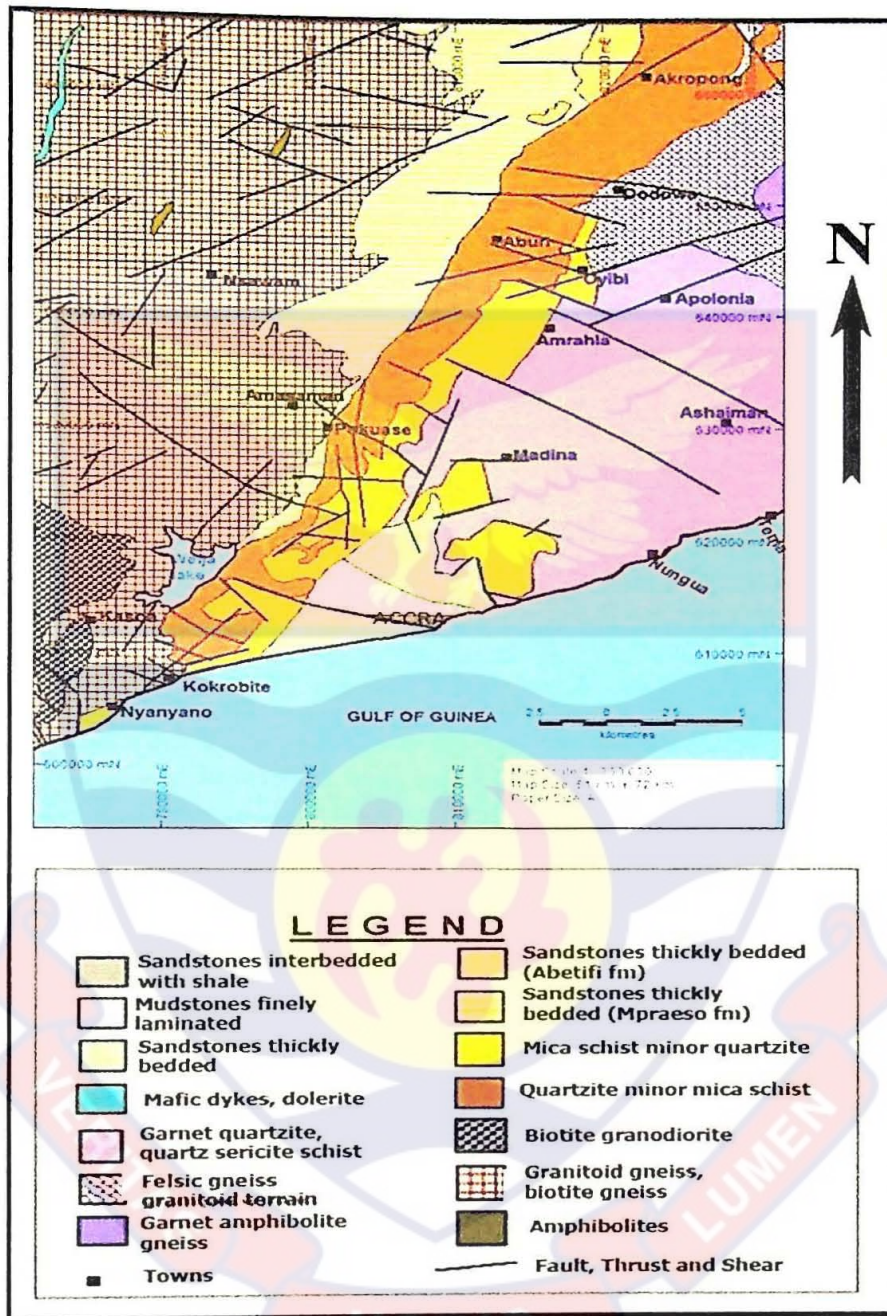
Figure 3.2: Geology of GAMA (Doku et. al., 2014)
