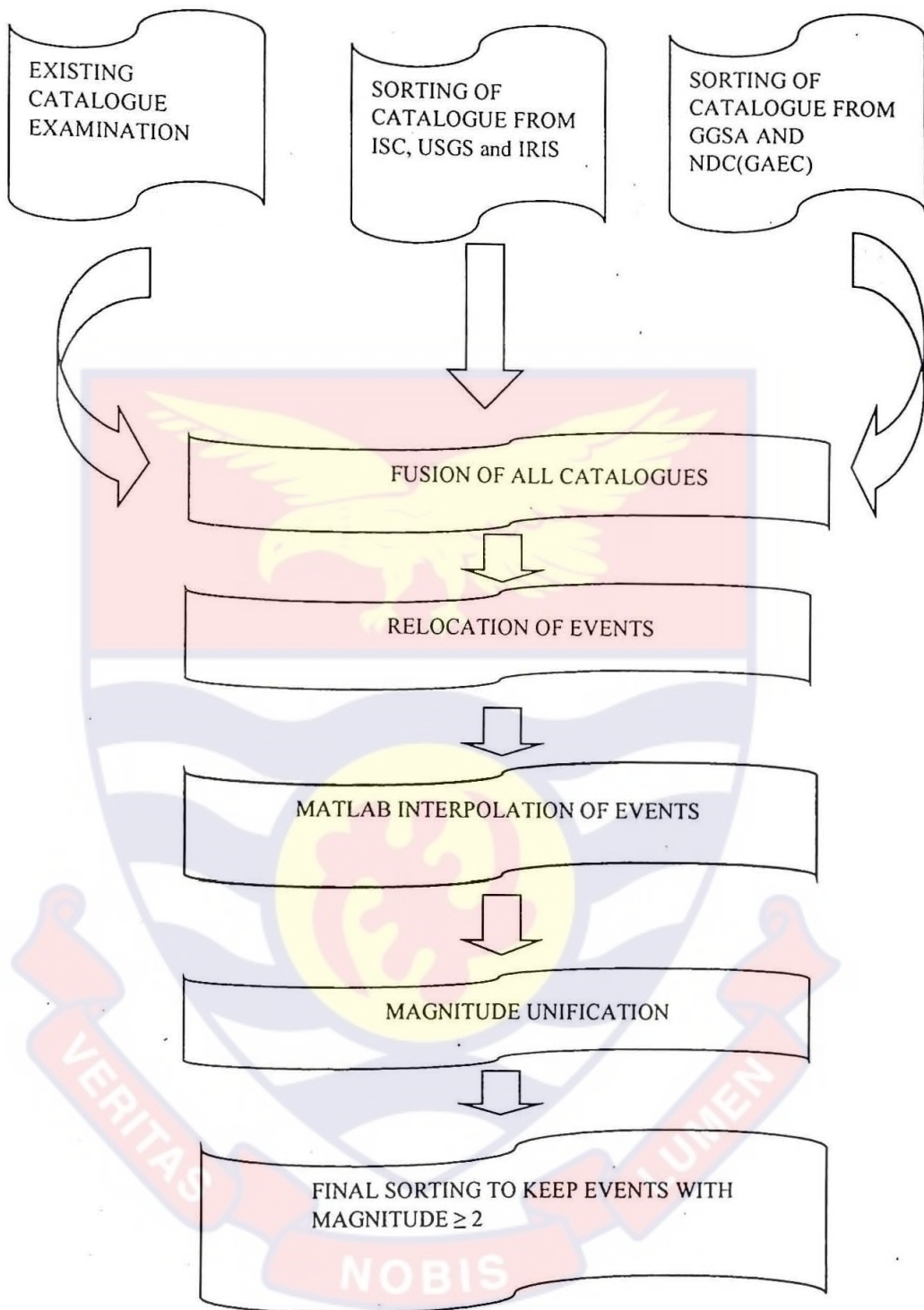
Figure 3.4: Seismicity Catalogue Flow Chart (Doku et. al., 2014)
