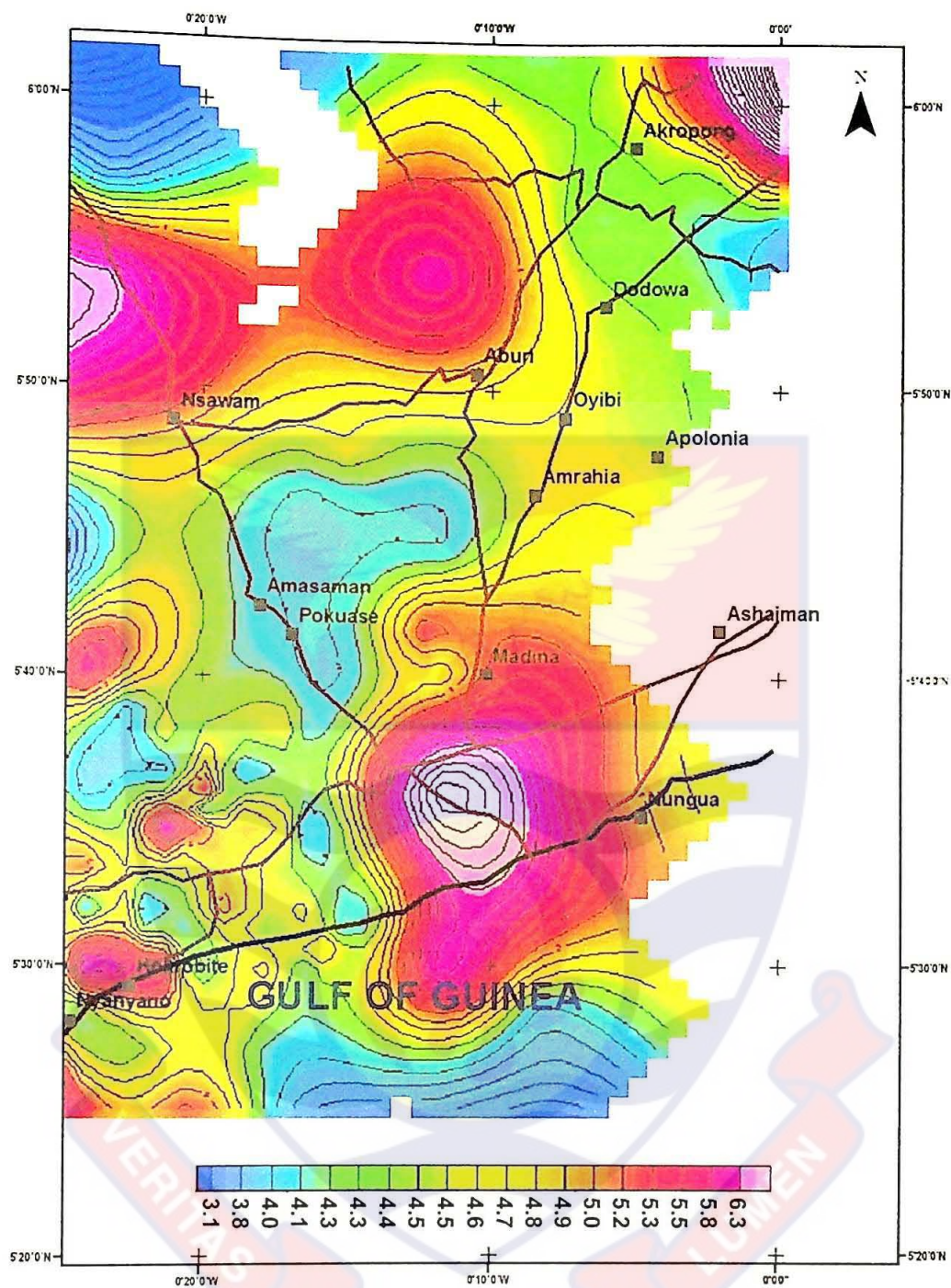
Figure 4.11: Isoseismal Map of GAMA
