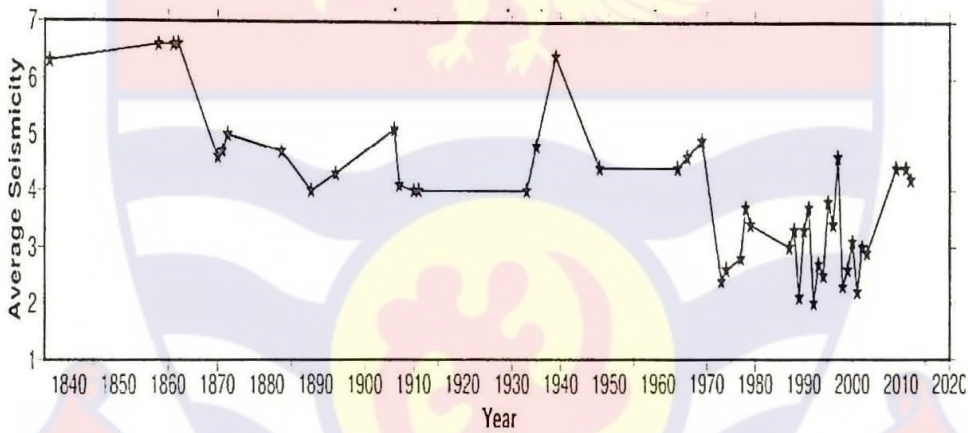
Figure 4.2: Plot of the Average Seismic Events from 1836-2018
