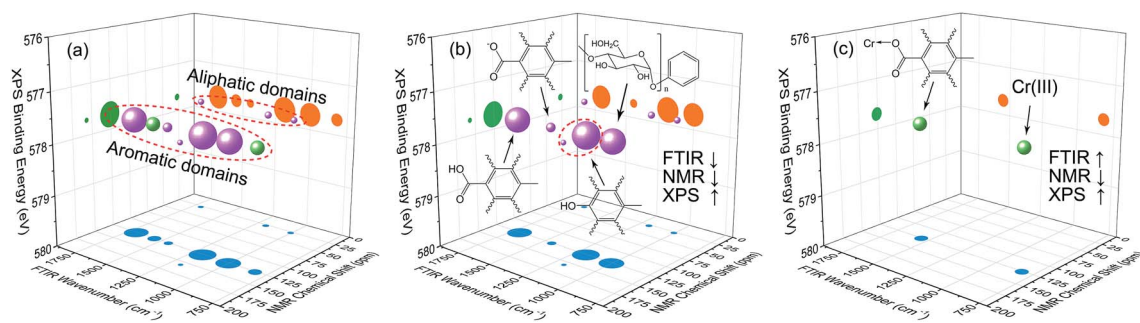
Fig. 8 Bubble diagram of three-dimensional hetero-spectral correlation analysis for FTIR, NMR, and XPS. \uparrow indicates the peak intensity increases with external perturbation, and \downarrow indicates the peak intensity decreases with external perturbation. Scaling factor \alpha = 0.75 .
