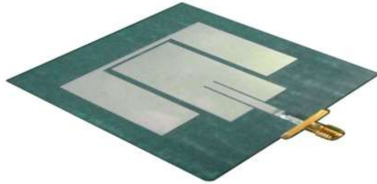
Figure 14: A photograph of a Microstrip antenna
