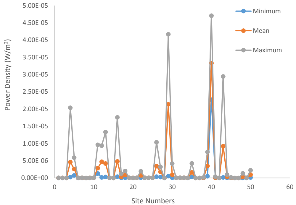
Figure 34: Graph of power density variation with site numbers
