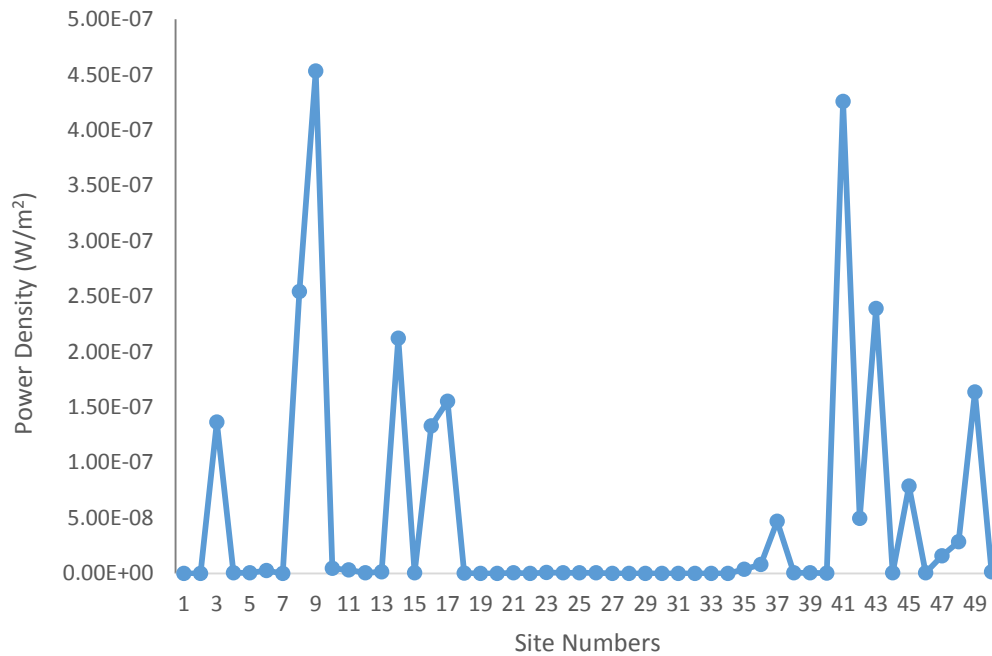
Figure 43: Graph of mean power density variation with site numbers
