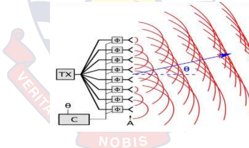
Figure 11: A schematic diagram of the Phased array antenna
