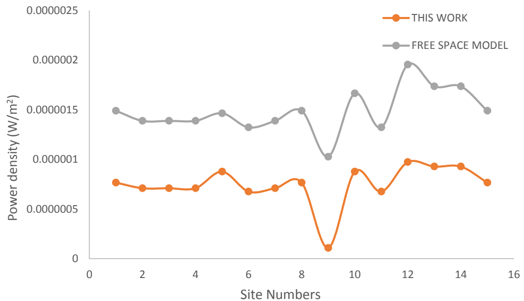
Figure 45: Comparison of results from this study with Friis model (Friis, 1946)
