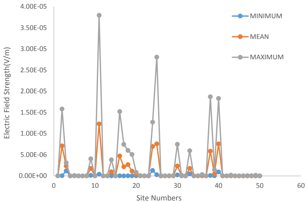
Figure 36: Graph of electric field strength variation with site numbers
