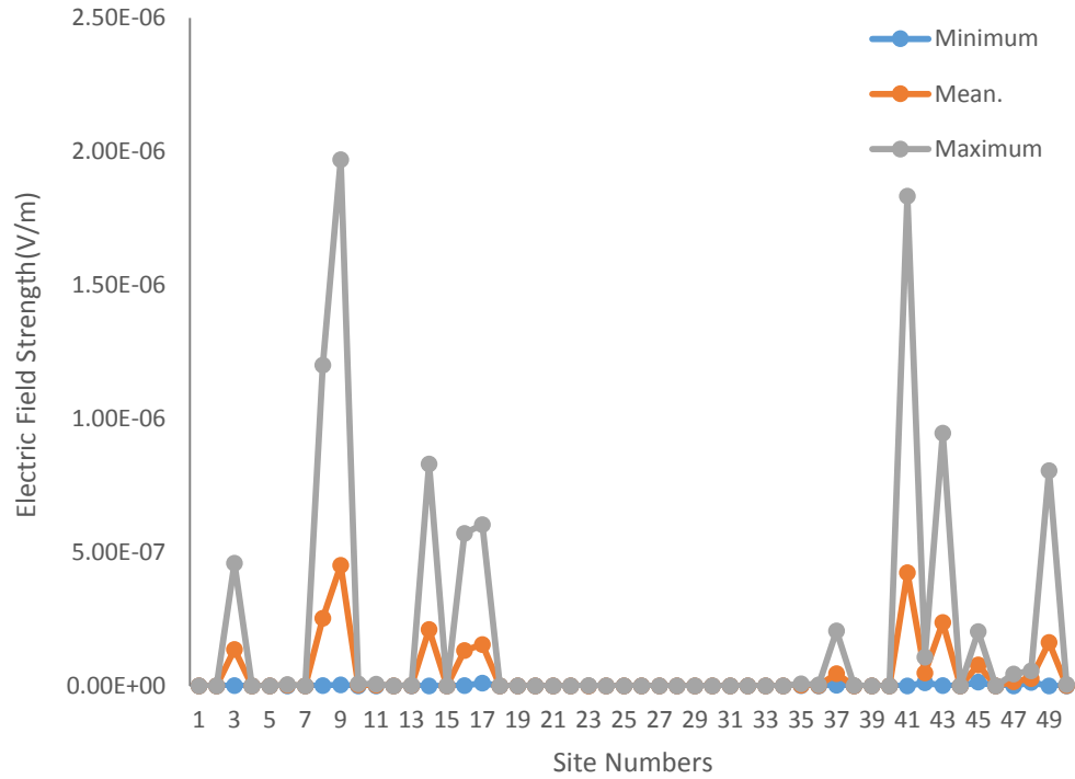
Figure 40: Graph of electric field strength variation with site numbers
