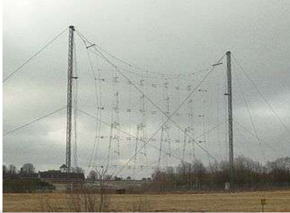
Figure 12: A photograph of a Curtain array antenna
