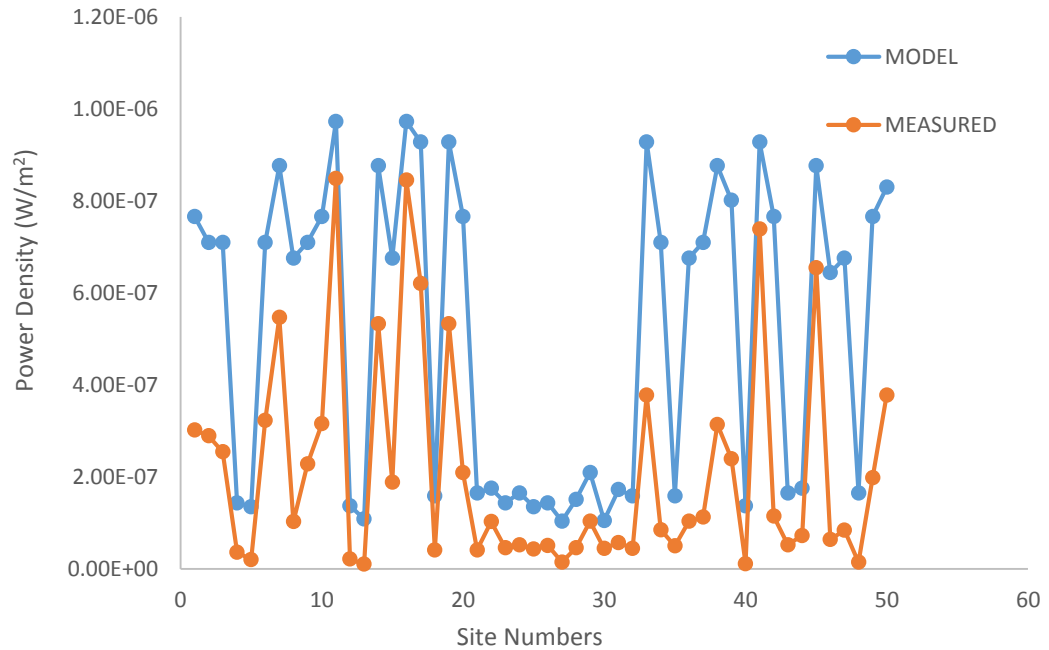
Figure 44: Verification of results from field measurement with the results from the model
