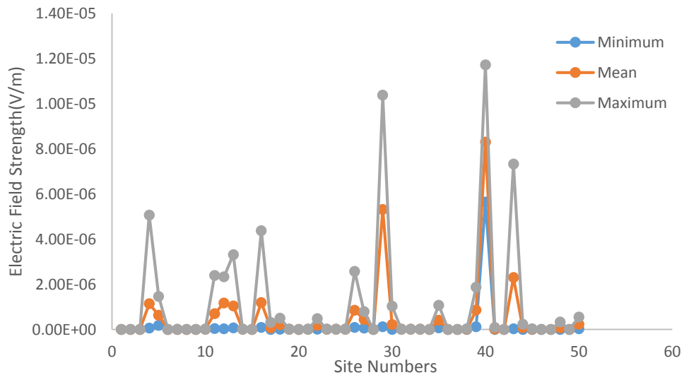
Figure 32: Graph of electric field strength variation with site numbers
