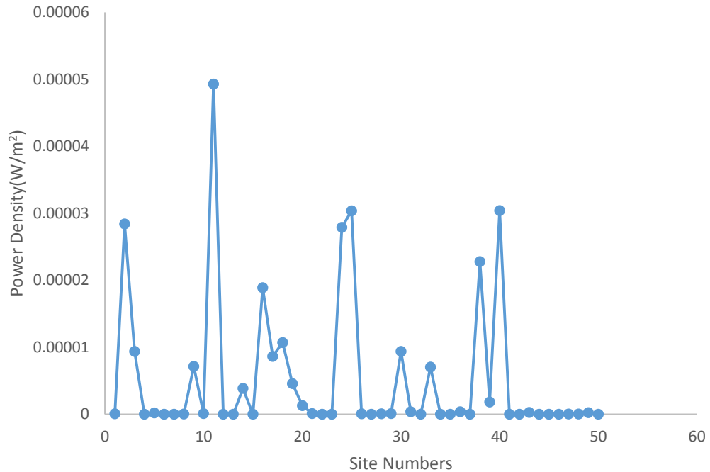
Figure 39: Graph of mean power density variation with site numbers
