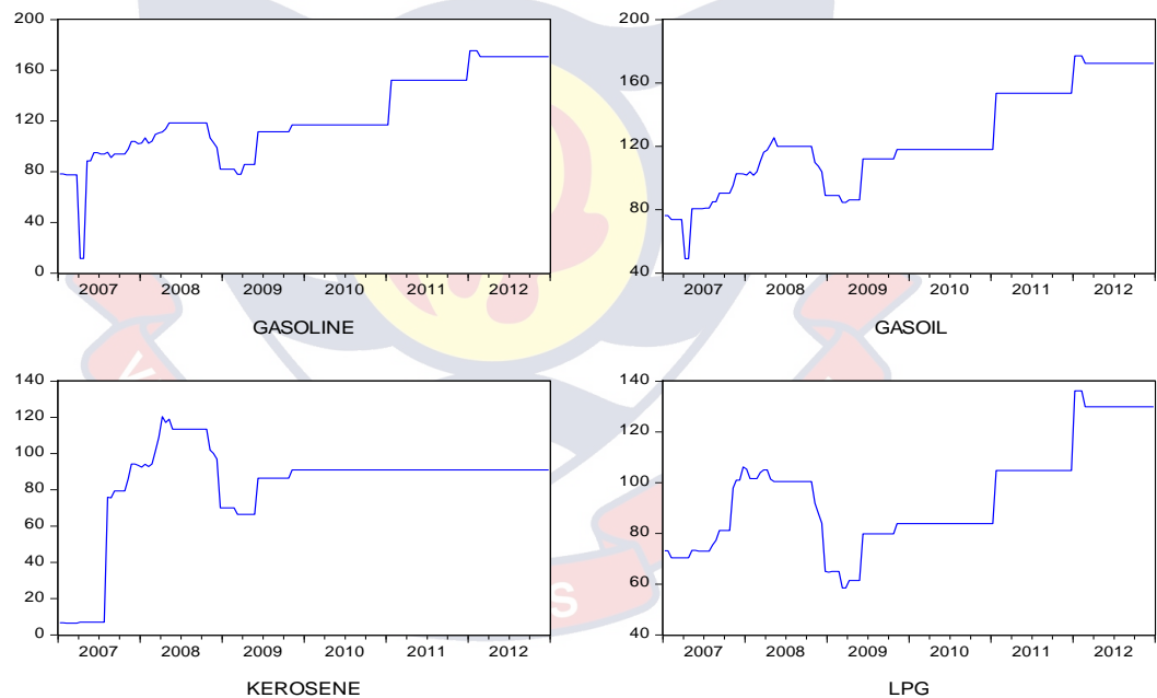
Figure 1: Time Series Plot of the Original Series
