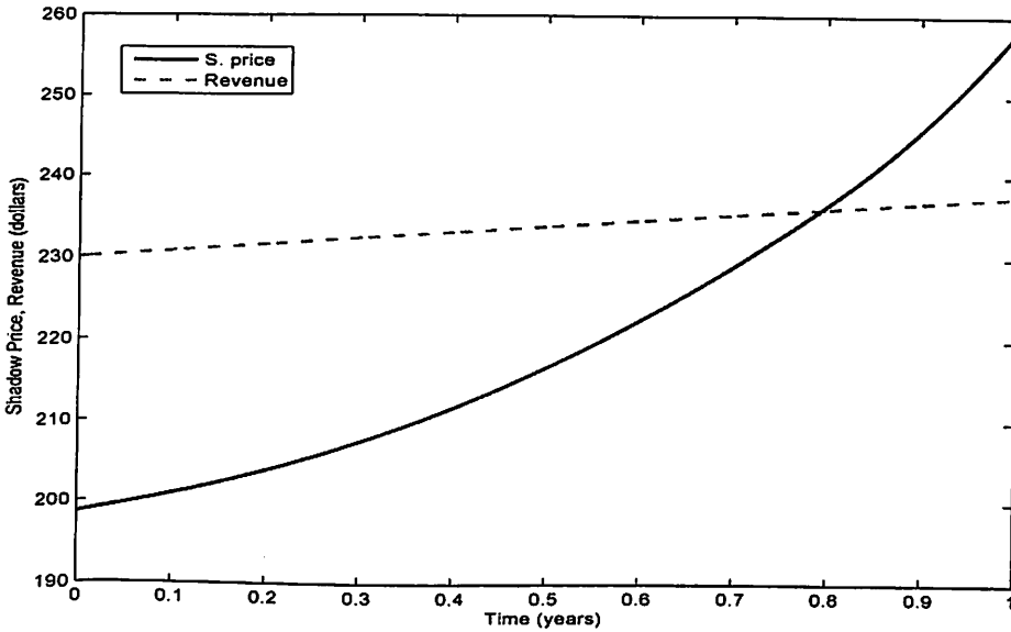
Figure 79: Shadow Price and Net Revenue for h_{max} = 250,000 and T = 1
