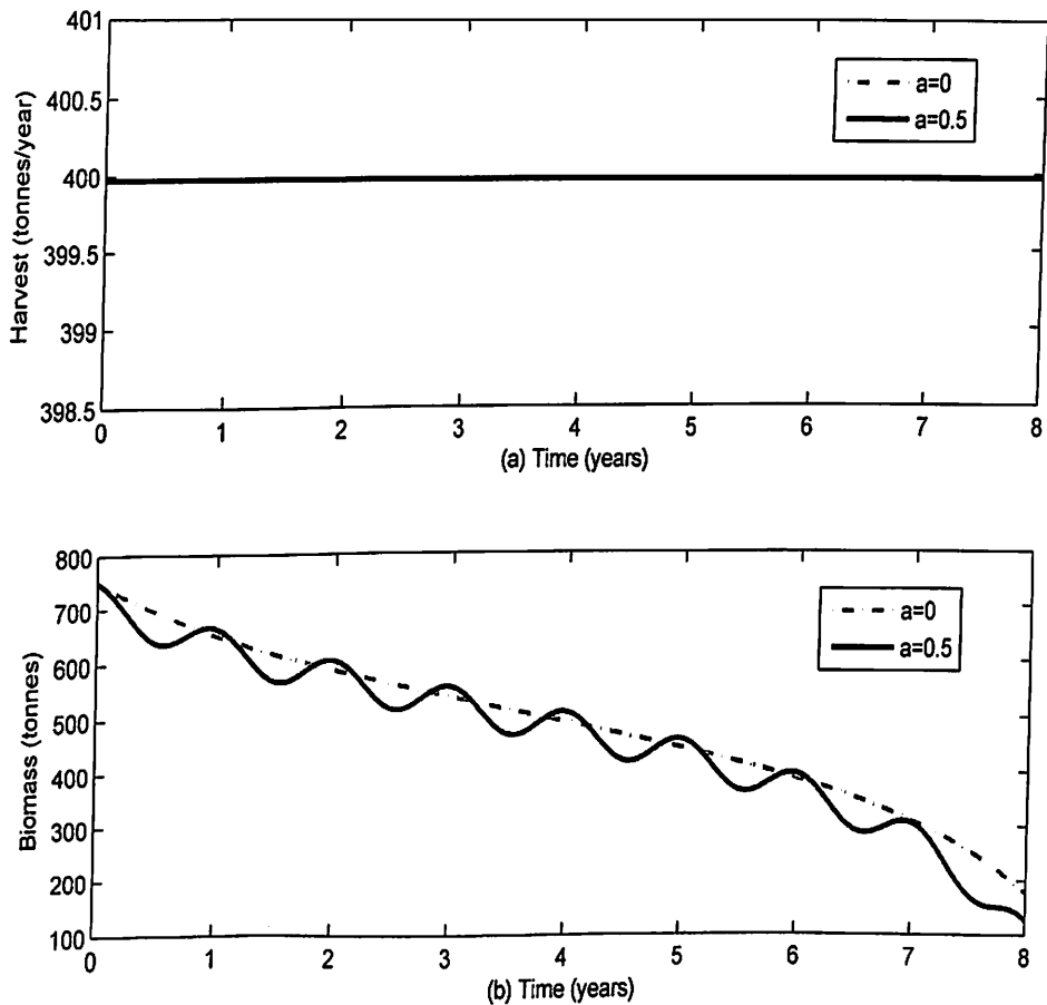
Figure 96: (a) Harvest and (b) Biomass Levels for h_{max} = 400,000 , x_0 = 750,000 , a = 0, 0.5 and T = 8
