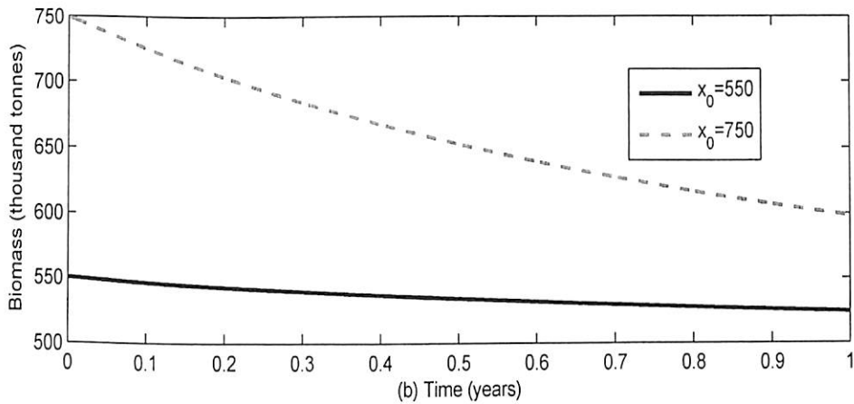
Figure 19: (a) Effort and (b) Biomass Levels for E_{max} = 394,444 , x_0 = 550,000 ; 750,000 and T = 1
