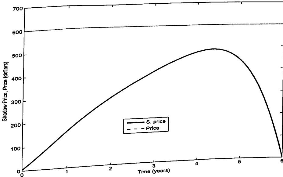
Figure 101: Shadow Price and Price for a = 200,000 , u_{max} = 0.5 and T = 6
