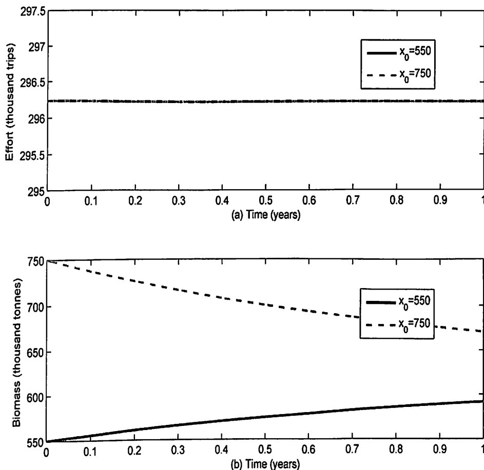
Figure 48: (a) Effort and (b) Biomass Levels for E_{max} = 296,380 ,
