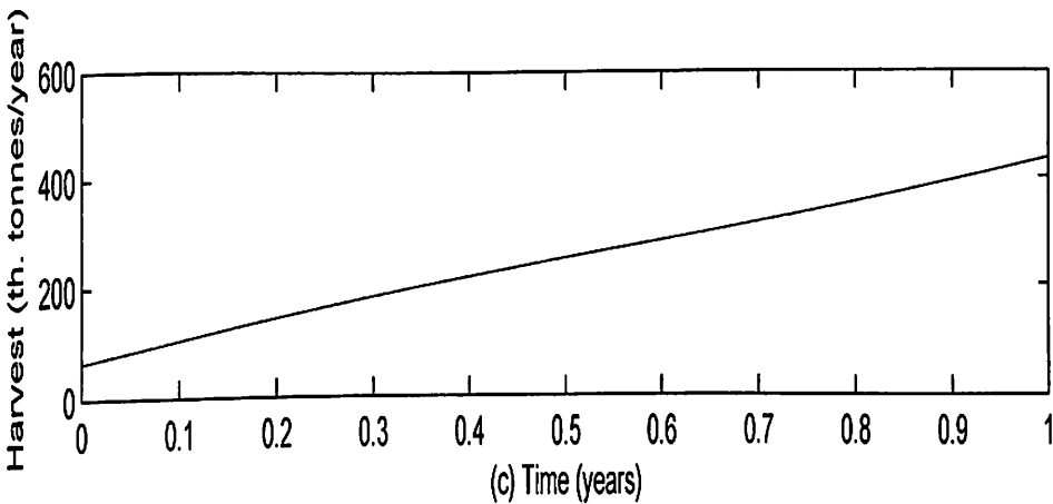
Figure 40: (a) Effort, (b) Biomass and (c) Harvest Levels for x_0 = 500,000 , z(T) = 250,000 , E_{max} = 800,000 and T = 1
