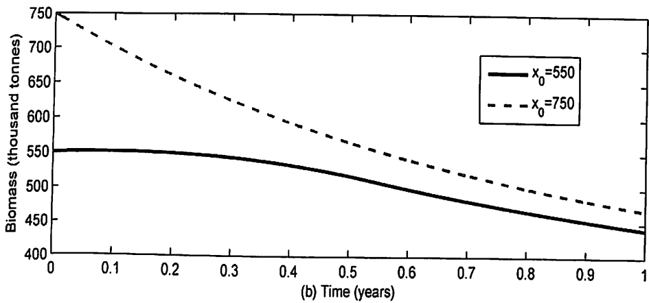
Figure 50: (a) Effort and (b) Biomass Levels for E_{max} = 592,761 , x_0 = 550,000 ; 750,000 and T = 1
