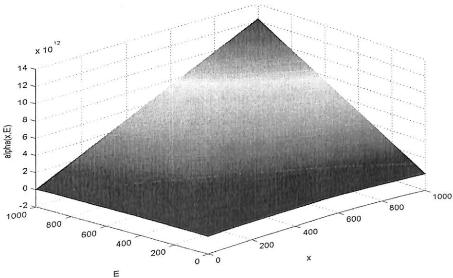
Figure 99: Determination of Sign of \alpha(x, E)
