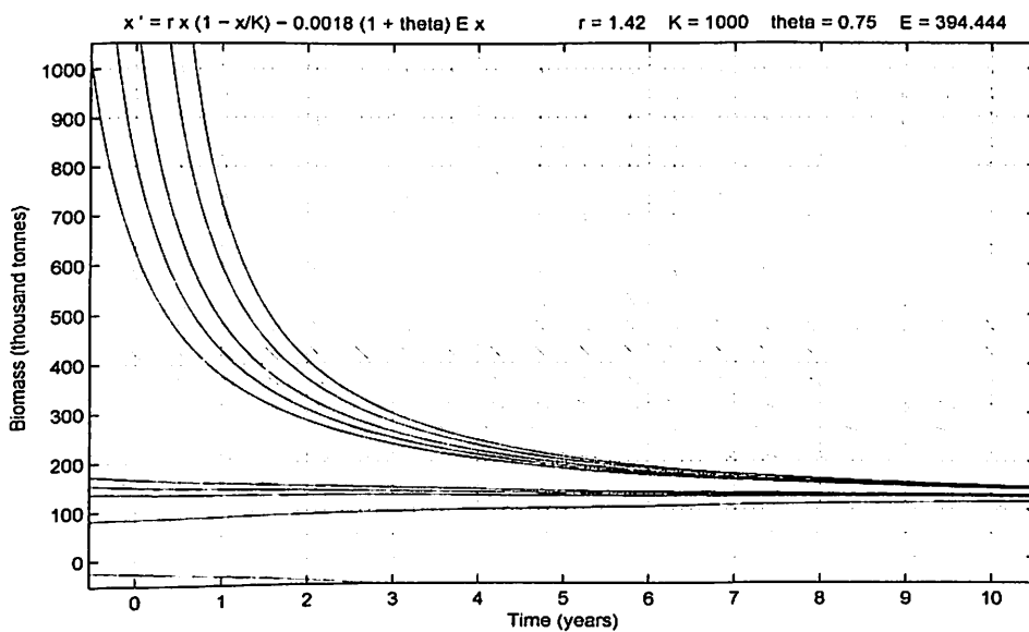
Figure 45: Solution Curves for E = 394.444 with \theta = 0.75
