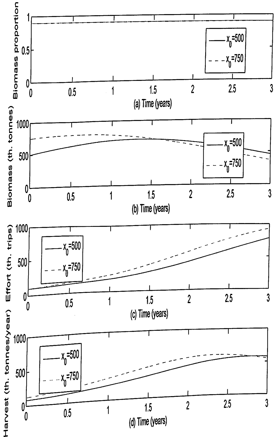
Figure 107: (a) Biomass Proportion, (b) Biomass, (c) Effort and (d) Harvest Levels for a = 200,000 , u_{max} = 0.9 and T = 3
