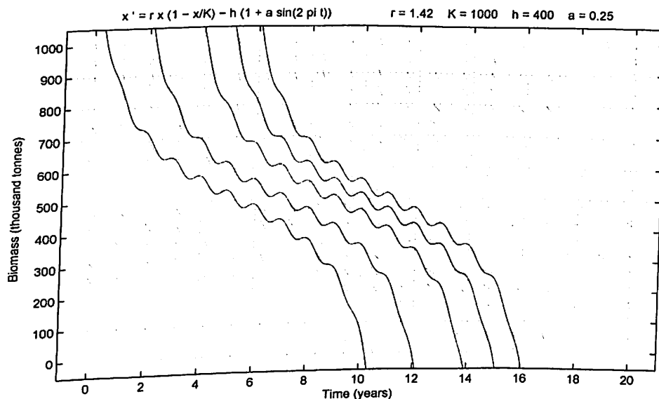
Figure 86: Periodic Cycles for h = 400,000
