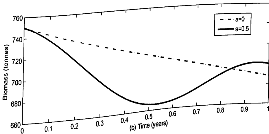
Figure 93: (a) Harvest and (b) Biomass Levels for h_{max} = 351,039 , a = 0, 0.5 and T = 1
