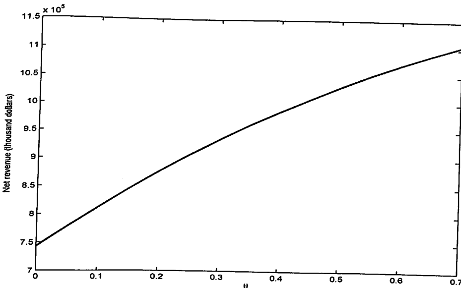
Figure 64: Net Revenue against \theta for \delta = 0.15 and T = 20
