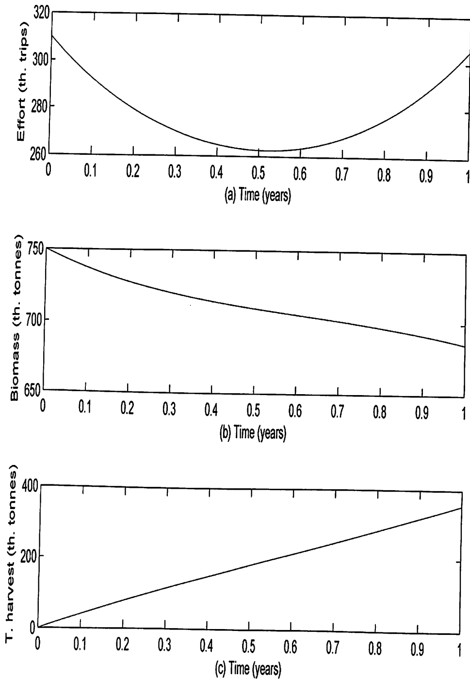
Figure 35: (a) Effort, (b) Biomass and (c) Total Harvest Levels for x_0 = 750,000 , z(T) = 355,000 , E_{max} = 800,000 and T = 1
