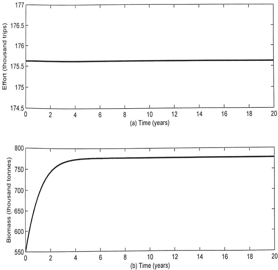
Figure 14: (a) Effort and (b) Biomass Levels for E_{max} = 175,664 , x_0 = 550,000 and T = 20
