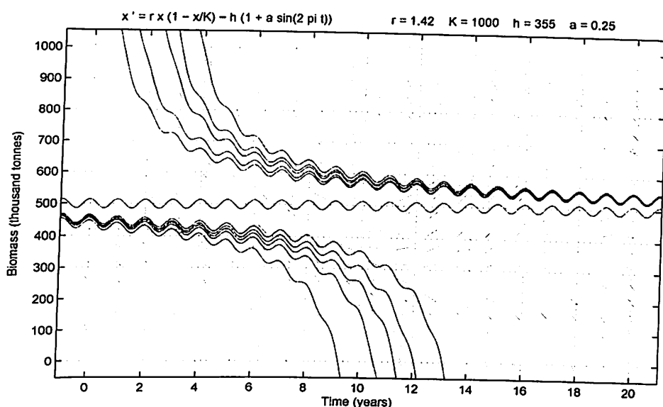
Figure 85: Periodic Cycles for h = 355,000
