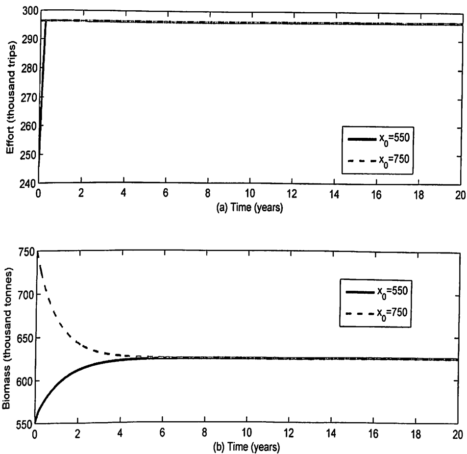
Figure 49: (a) Effort and (b) Biomass Levels for E_{max} = 296,380 ,
