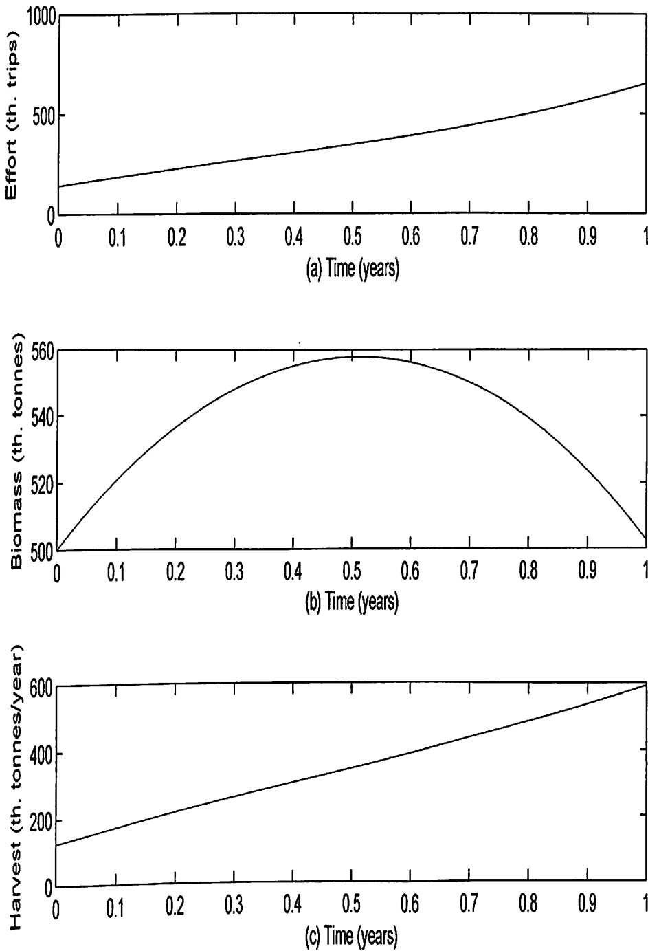
Figure 41: (a) Effort, (b) Biomass and (c) Harvest Levels for x_0 = 500,000 , z(T) = 350,000 , E_{max} = 800,000 and T = 1
