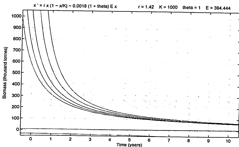
Figure 46: Solution Curves for E = 394.444 with \theta = 1
