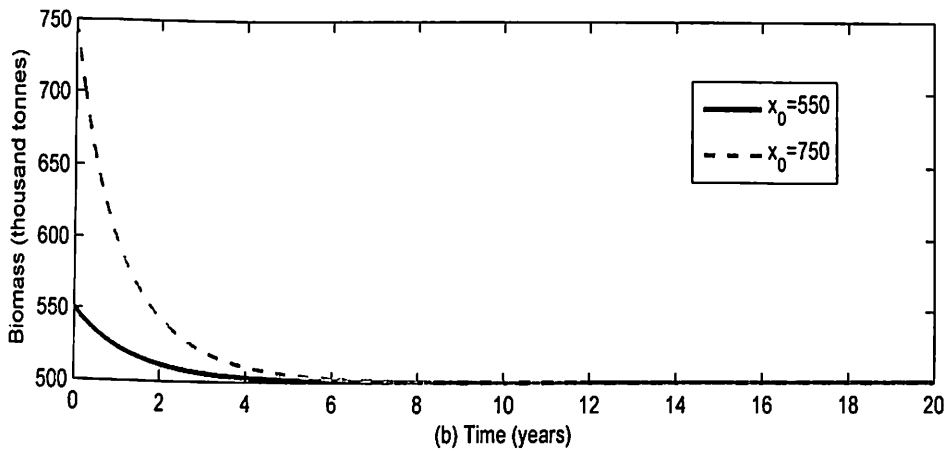
Figure 20: (a) Effort and (b) Biomass Levels for E_{max} = 394,444 , x_0 = 550,000 ; 750,000 and T = 20
