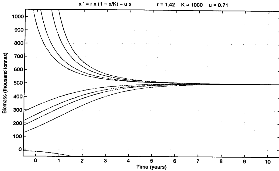
Figure 25: Solution Curves for u = 0.71
