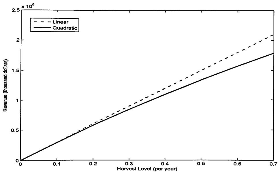
Figure 28: Linear and Quadratic Revenues
