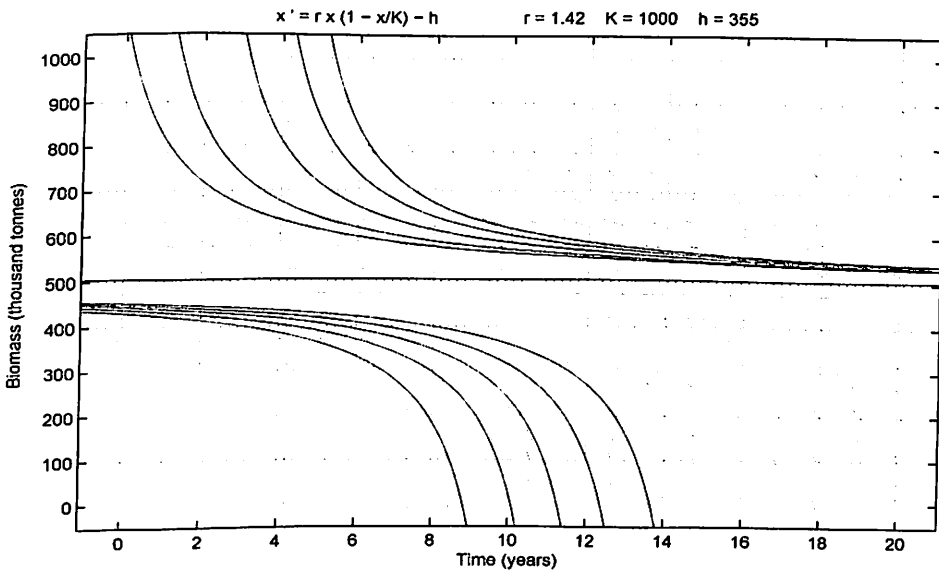
Figure 67: Solution Curves for h = 355,000
