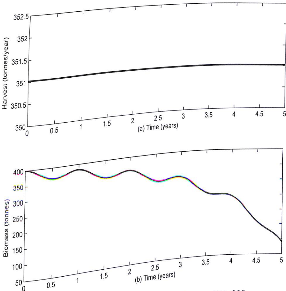
Figure 91: (a) Harvest and (b) Biomass Levels for h_{max} = 351,039 , x_0 = 400,000 , a = 0.25 and T = 5
