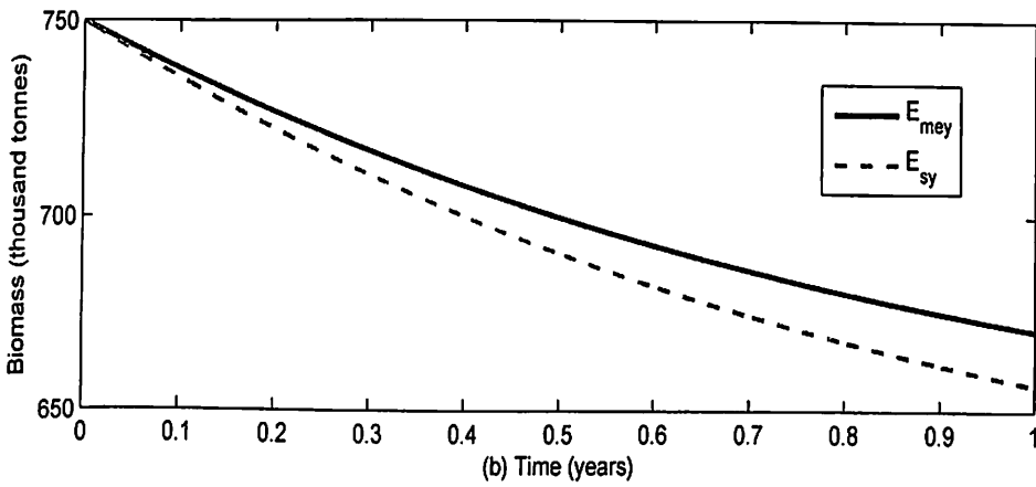
Figure 52: (a) Effort and (b) Biomass levels for E_{max} = 296,380; 315,000 , x_0 = 750,000 and T = 1
