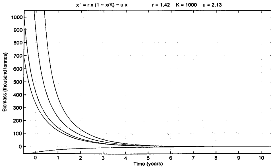
Figure 27: Solution Curves for u = 2.13
