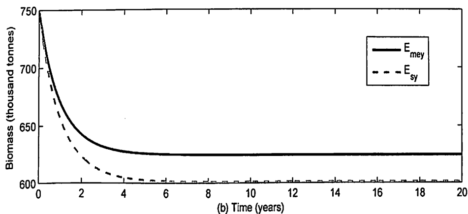
Figure 53: (a) Effort and (b) Biomass Levels for E_{max} = 296,380; 315,000 , x_0 = 750,000 and T = 20
