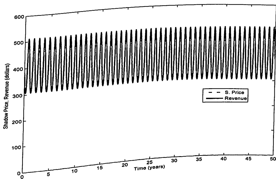
Figure 89: Shadow Price and Net Revenue for h_{max} = 351,039 , x_0 = 750,000 , a = 0.25 and T = 50
