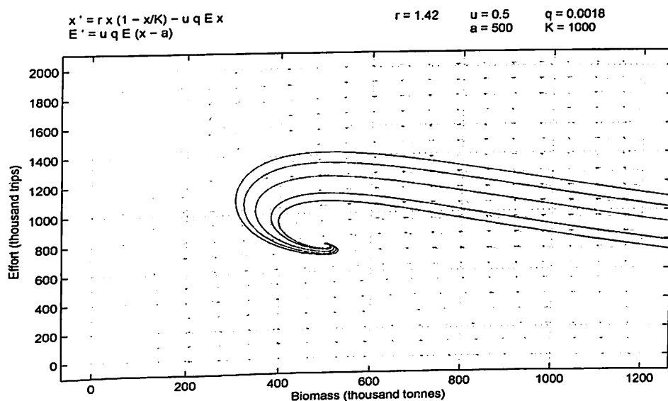
Figure 98: Phase-Plane Portrait for a = 500,000 and u = 0.5
