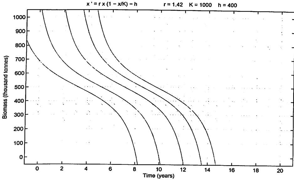
Figure 68: Solution Curves for h = 400,000
