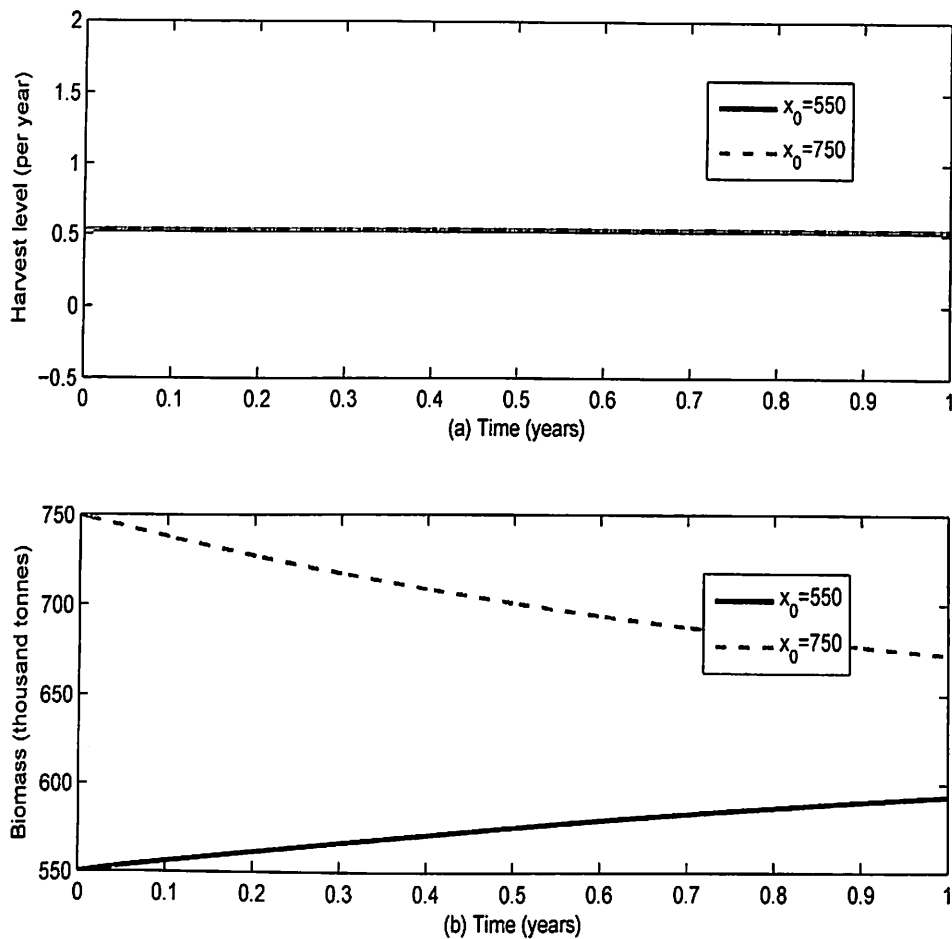
Figure 29: (a) Harvest and (b) Biomass Levels for x_0 = 550,000; 750,000 ,
