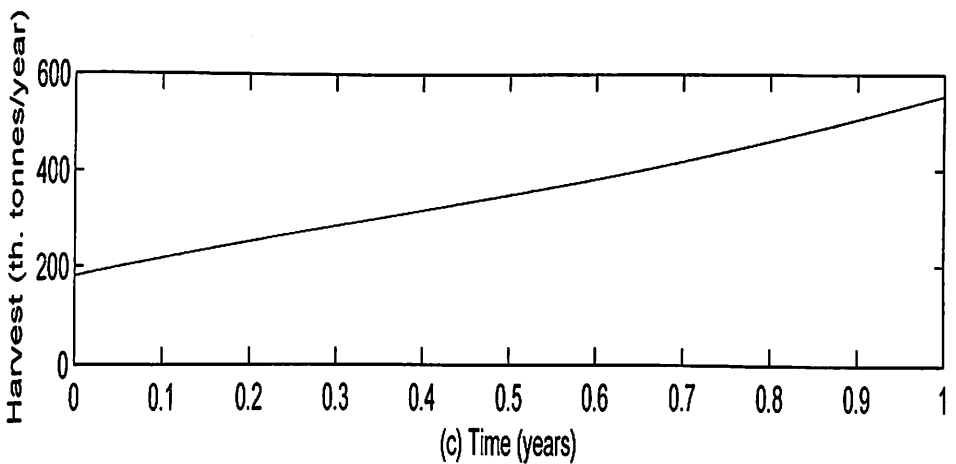
Figure 37: (a) Effort, (b) Biomass and (c) Harvest Levels for x_0 = 550,000 , z(T) = 355,000 , E_{max} = 800,000 and T = 1
