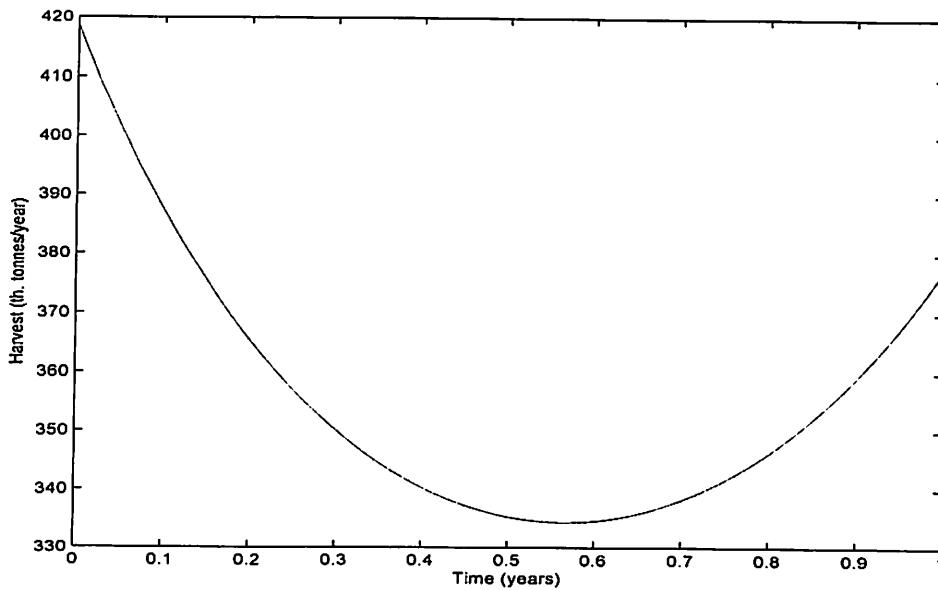
Figure 36: Harvest Level for x_0 = 750,000 , z(T) = 355,000 , E_{max} = 800,000 and T = 1
