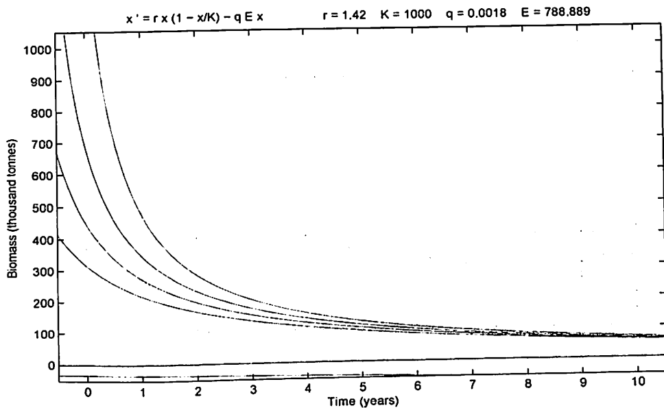
Figure 5: Solution Curves for E = 788,889
