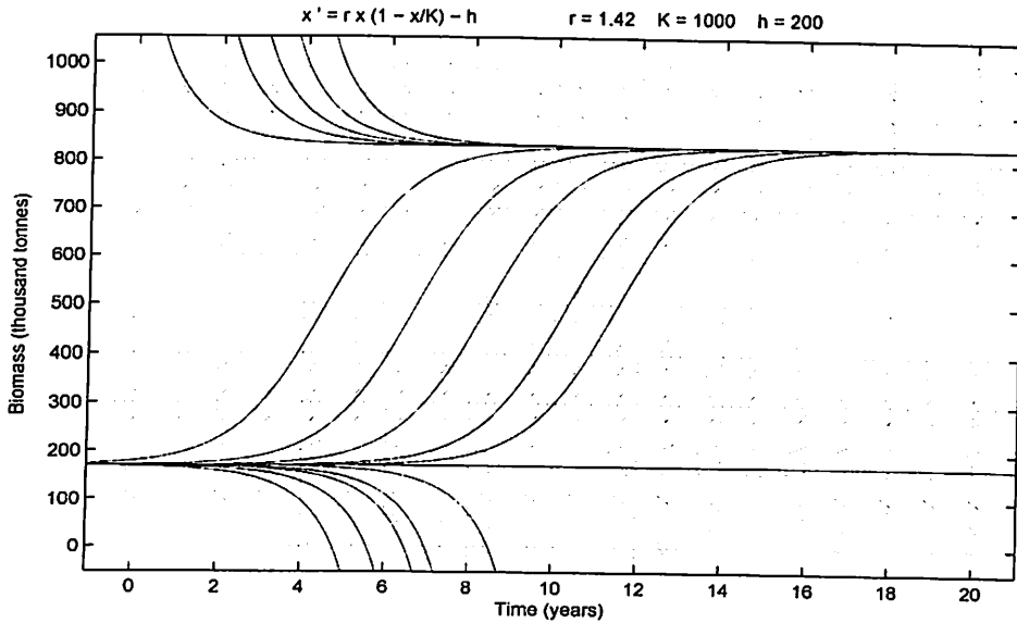
Figure 66: Solution Curves for h = 200,000
