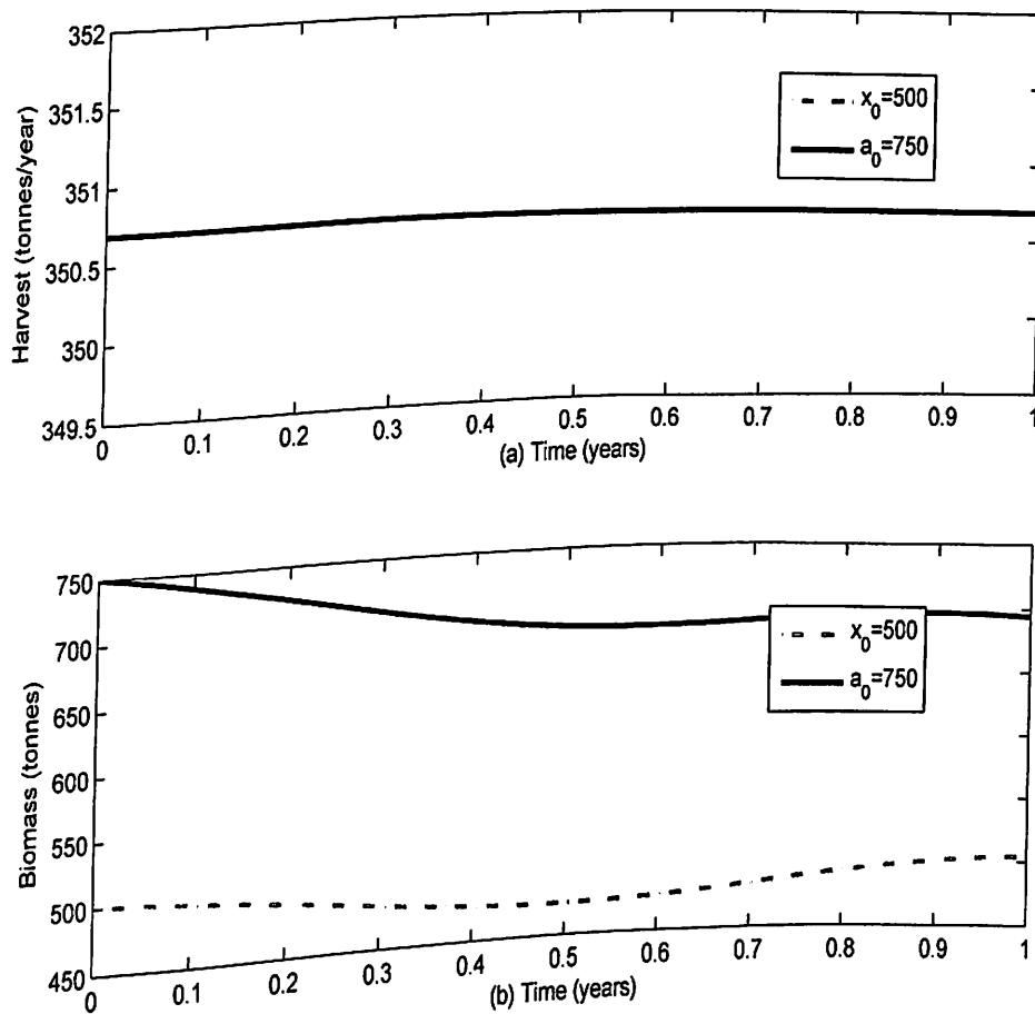
Figure 88: (a) Harvest and (b) Biomass Levels for h_{max} = 351,039 , x_0 = 500,000; 750,000 , a = 0.25 and T = 1
