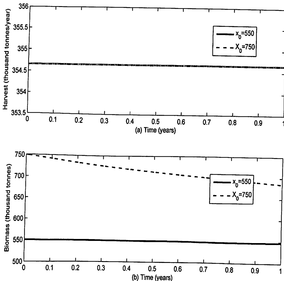
Figure 73: (a) Harvest and (b) Biomass Levels for h_{max} = 355,000 , x_0 = 550,000; 750,000 and T = 1
