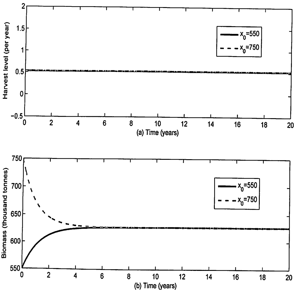
Figure 30: (a) Harvest and (b) Biomass Levels for x_0 = 550,000; 750,000 , u_{max} = 0.53 and T = 20
