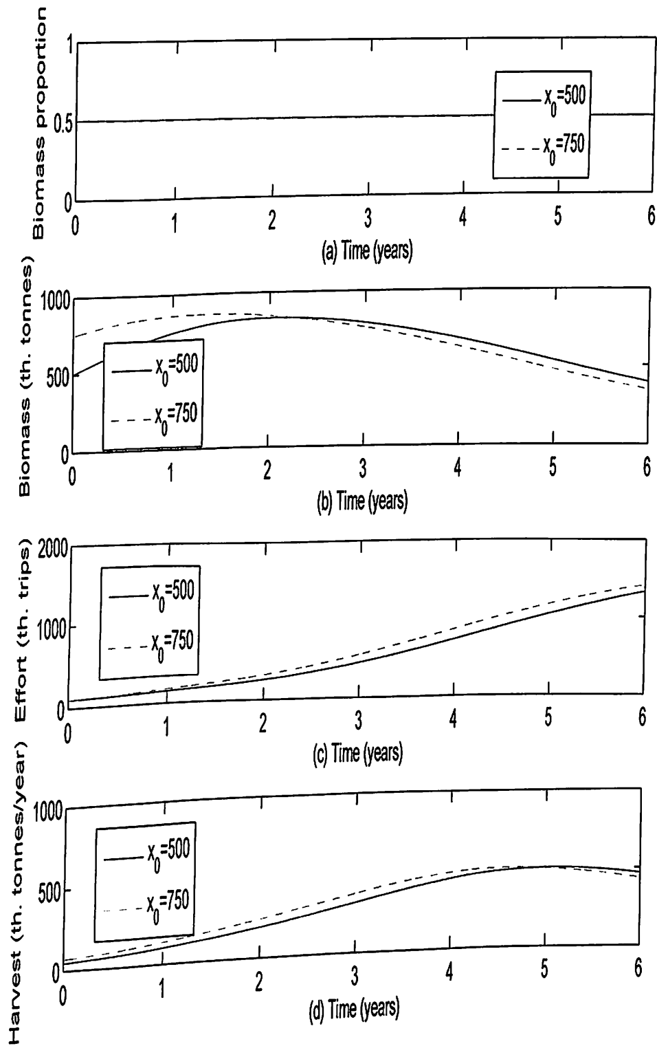
Figure 102: (a) Biomass Proportion, (b) Biomass, (c) Effort and (d) Harvest Levels for a = 200,000 , u_{max} = 0.5 and T = 6
