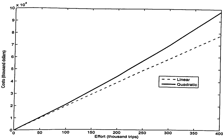
Figure 47: Linear and Quadratic Costs
