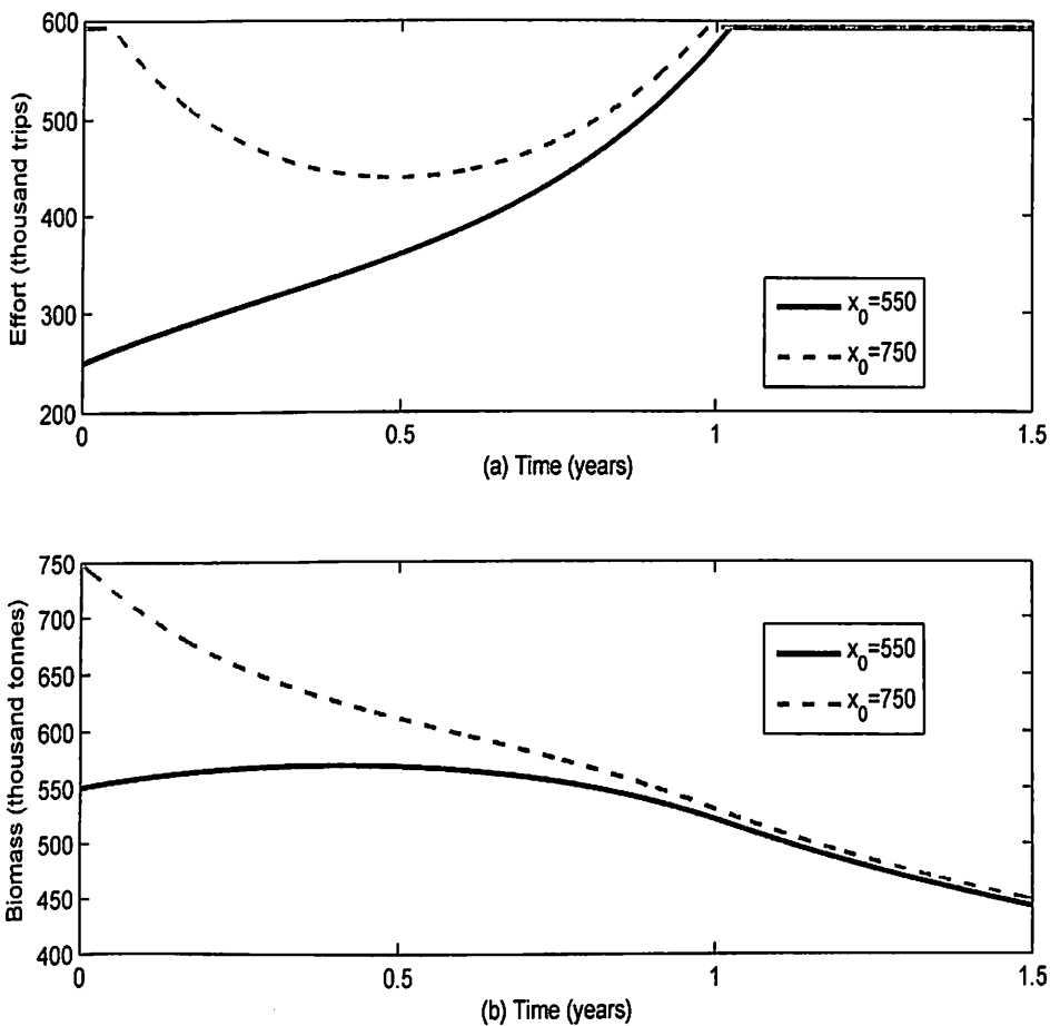
Figure 51: (a) Effort and (b) Biomass Levels for E_{max} = 592,761 , x_0 = 550,000 ; 750,000 and T = 1.5
