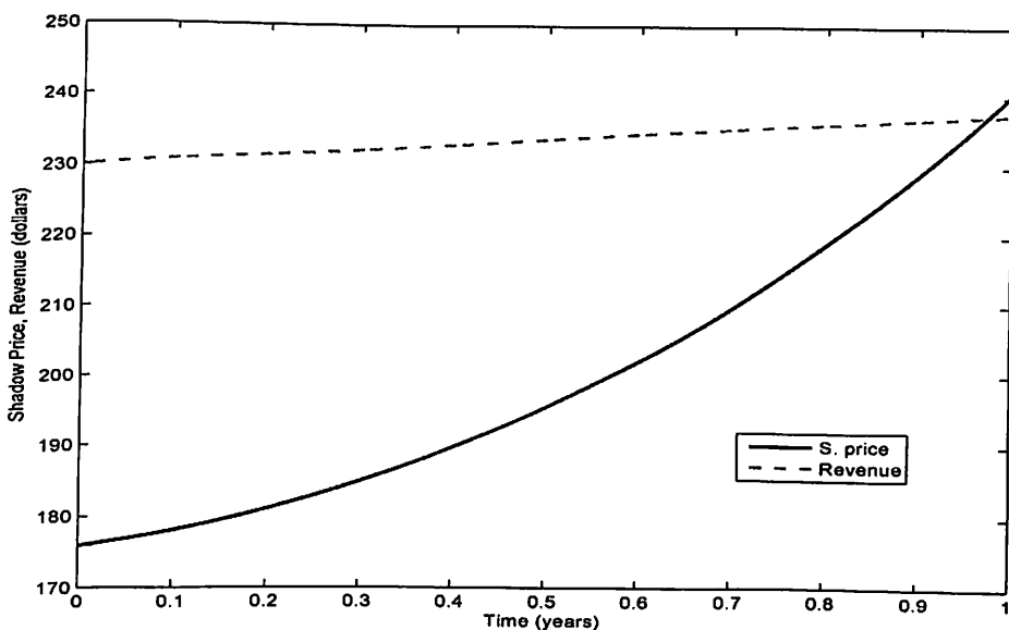
Figure 77: Shadow Price and Net Revenue for h_{max} = 200,000 and T = 1
