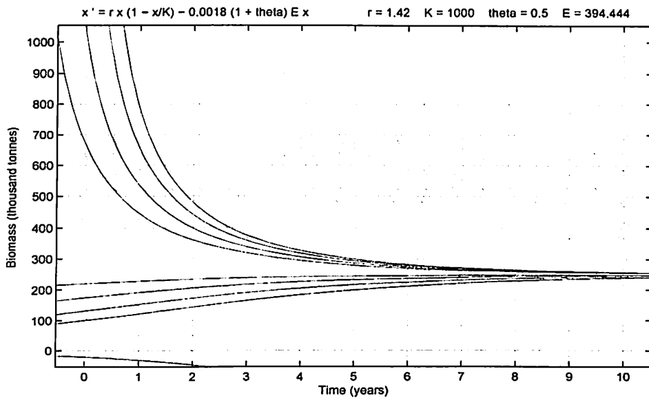
Figure 44: Solution Curves for E = 394.444 with \theta = 0.5
