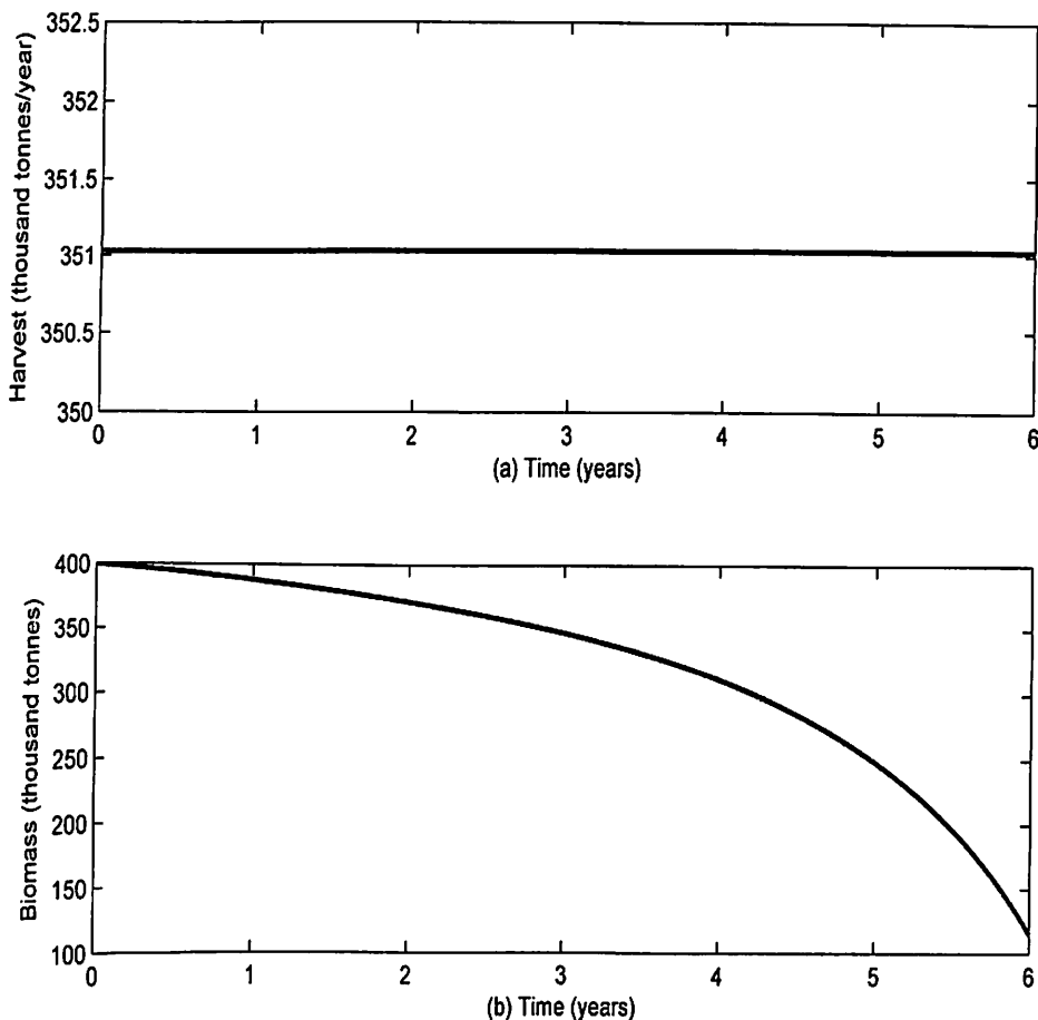
Figure 71: (a) Harvest and (b) Biomass Levels for h_{max} = 351,039 ,
