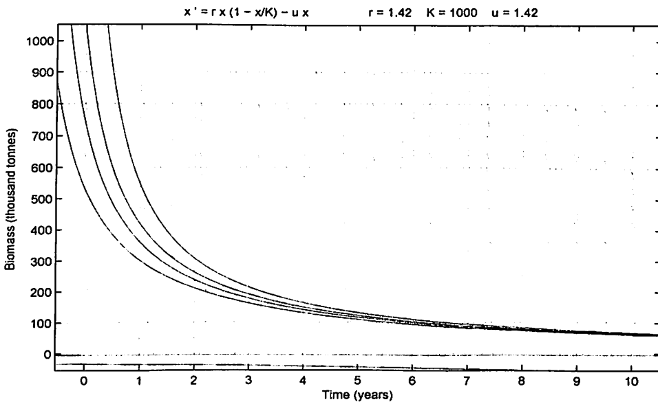
Figure 26: Solution Curves for u = 1.42
