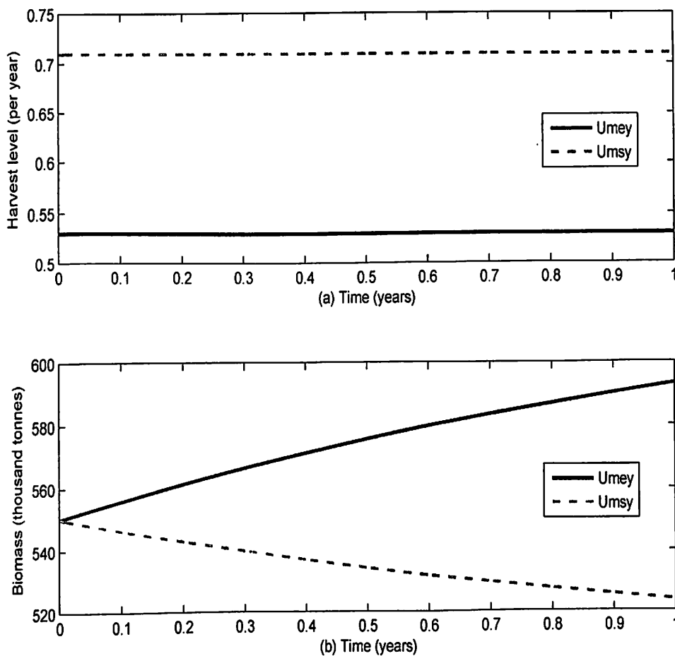
Figure 33: (a) Harvest and (b) Biomass Levels for x_0 = 550,000 ,
