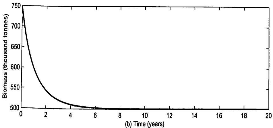
Figure 18: (a) Effort and (b) Biomass Levels for E_{max} = 394,444 , x_0 = 750,000 and T = 20
