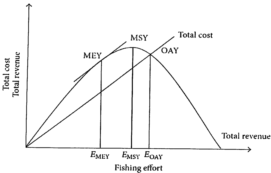
Figure 1: The Static Gordon-Schaefer Model
