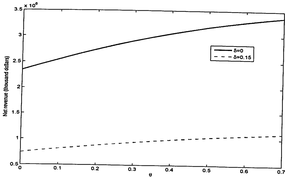
Figure 65: Net Revenue against \theta for \delta = 0, 0.15 and T = 20
