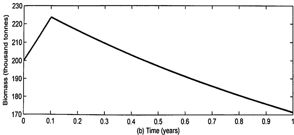
Figure 24: (a) Effort and (b) Biomass Levels for E_{max} = 800,000 , x_0 = 200,000 and T = 1
