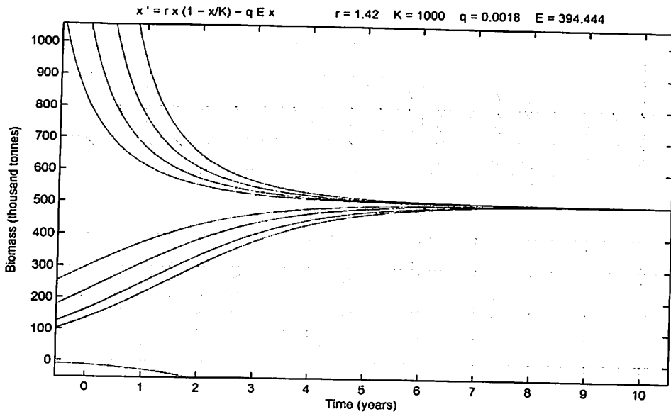
Figure 42: Solution Curves for E = 394.444
