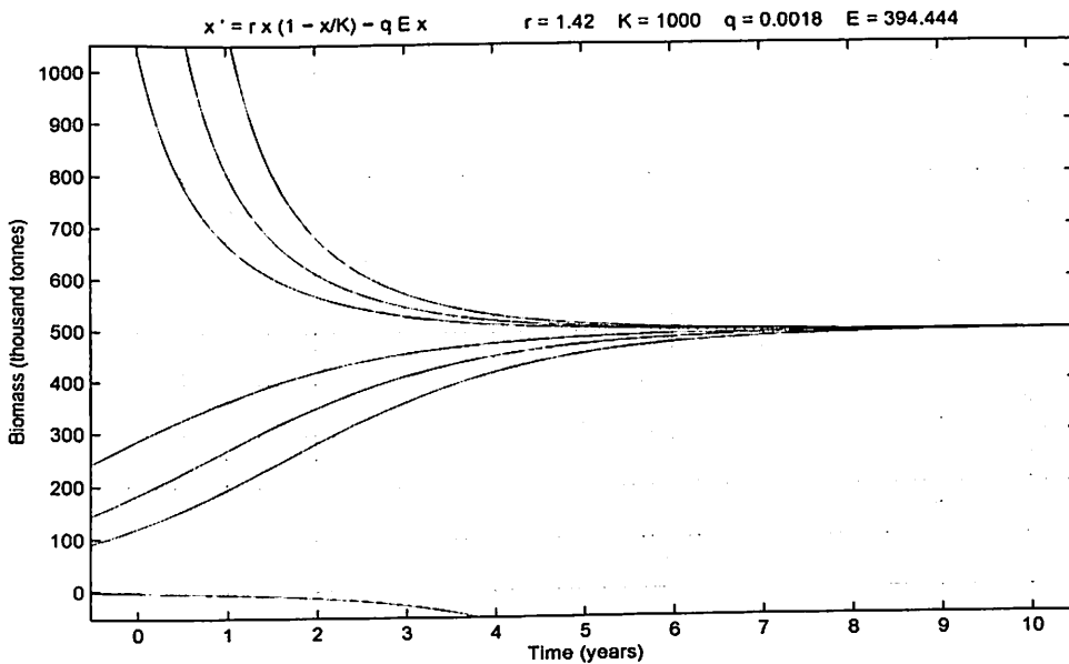
Figure 3: Solution Curves for E = 394,444
