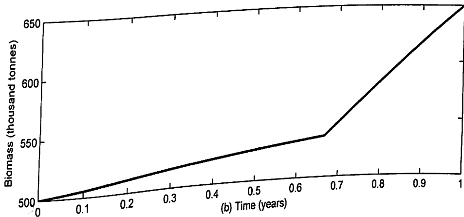
Figure 82: (a) Harvest Strategy and (b) Biomass Level for h_{max} = 300,000 and T = 1
