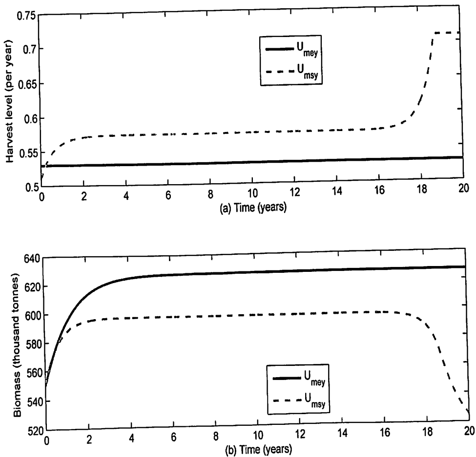
Figure 34: (a) Harvest and (b) Biomass Levels for x_0 = 550,000 ,
