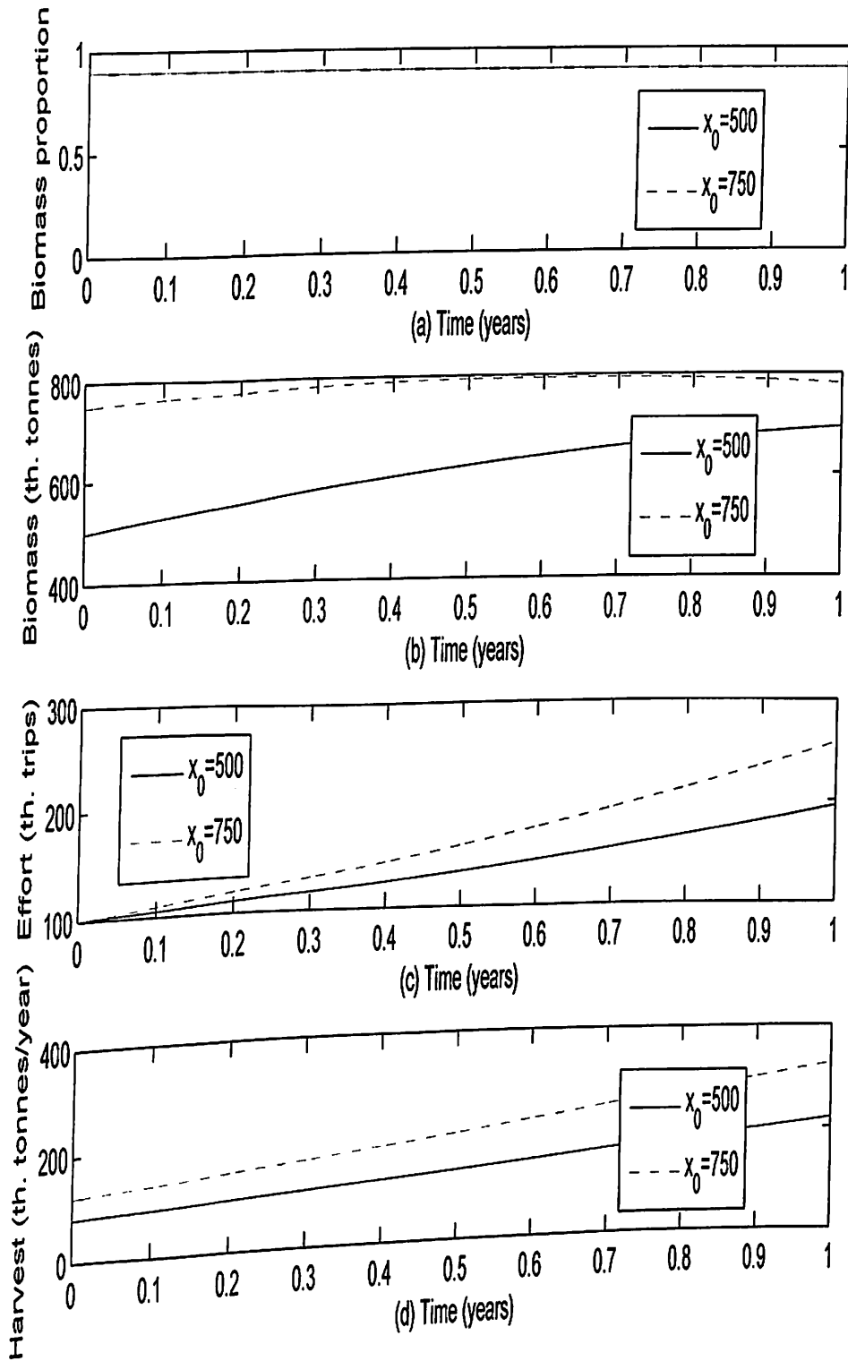
Figure 106: (a) Biomass Proportion, (b) Biomass, (c) Effort and (d) Harvest Levels for a = 200,000 , u_{max} = 0.9 and T = 1
