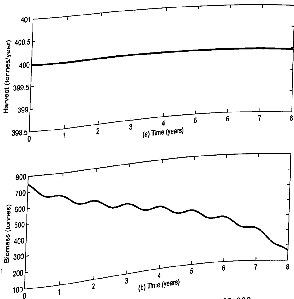
Figure 92: (a) Harvest and (b) Biomass Levels for h_{max} = 400,000 , x_0 = 750,000 , a = 0.25 and T = 8
