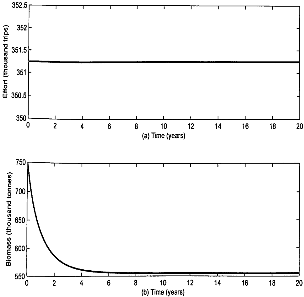
Figure 10: (a) Effort and (b) Biomass Levels for E_{max} = 351,328 , x_0 = 750,000 and T = 20
