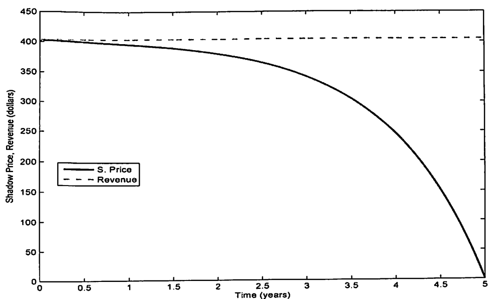
Figure 12: Shadow Price and Net Revenue for E_{max} = 351,328 , x_0 = 550,000 and T = 5
