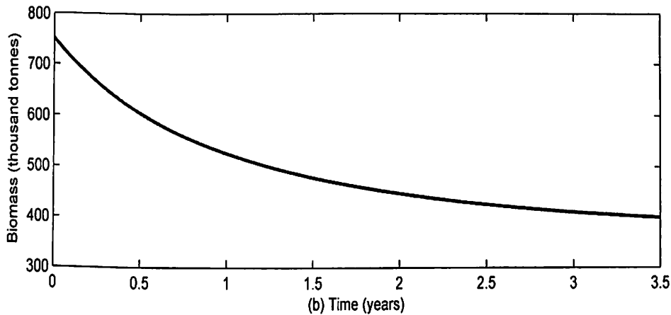
Figure 21: (a) Effort and (b) Biomass Levels for E_{max} = 500,000 , x_0 = 750,000 and T = 3.5
