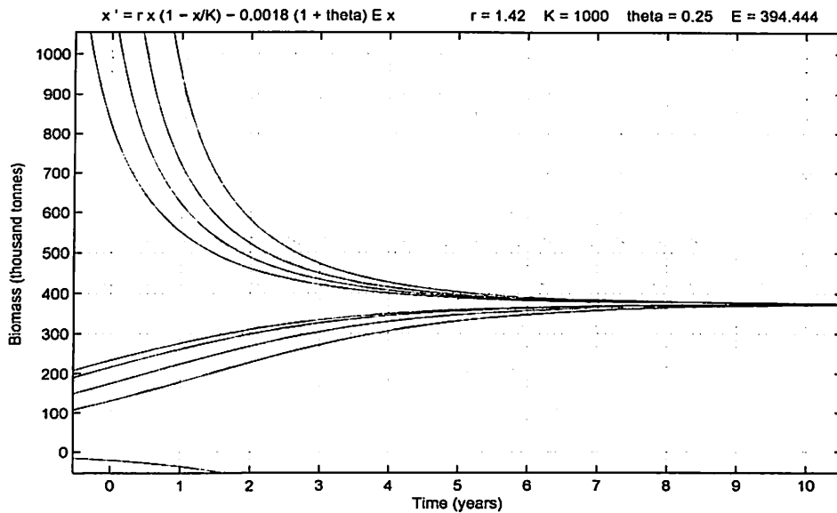
Figure 43: Solution Curves for E = 394,444 with \theta = 0.25
