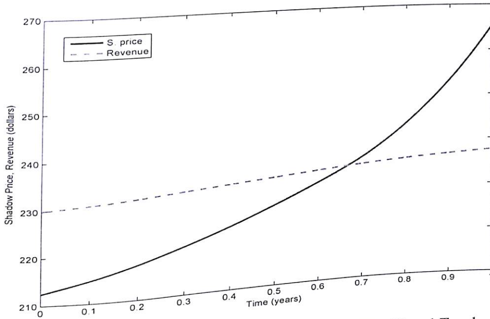
Figure 81: Shadow Price and Net Revenue for h_{max} = 300,000 and T = 1
