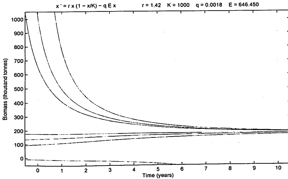
Figure 4: Solution Curves for E = 646,450
