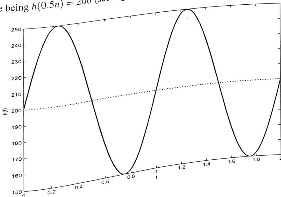
Figure 83: Periodic Rate Harvesting
