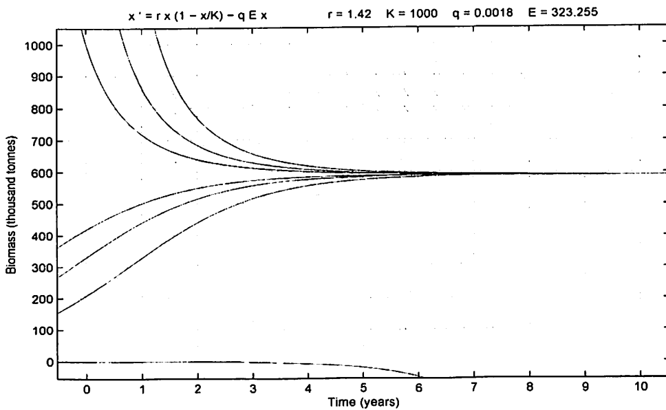
Figure 2: Solution Curves for E = 323,255
