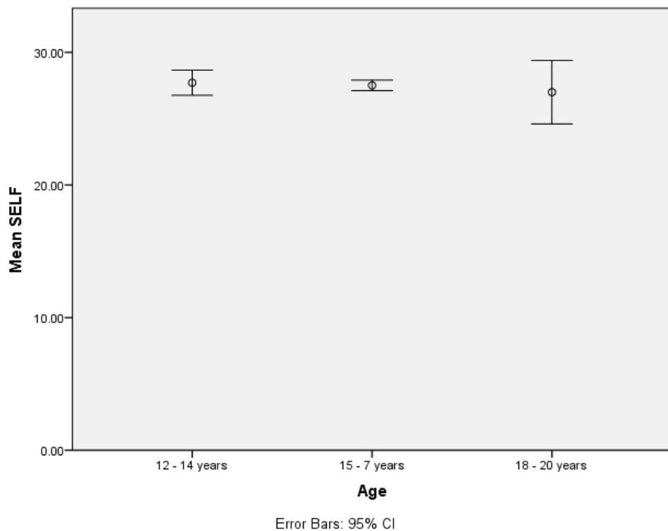
Figure 1: Means Plots
