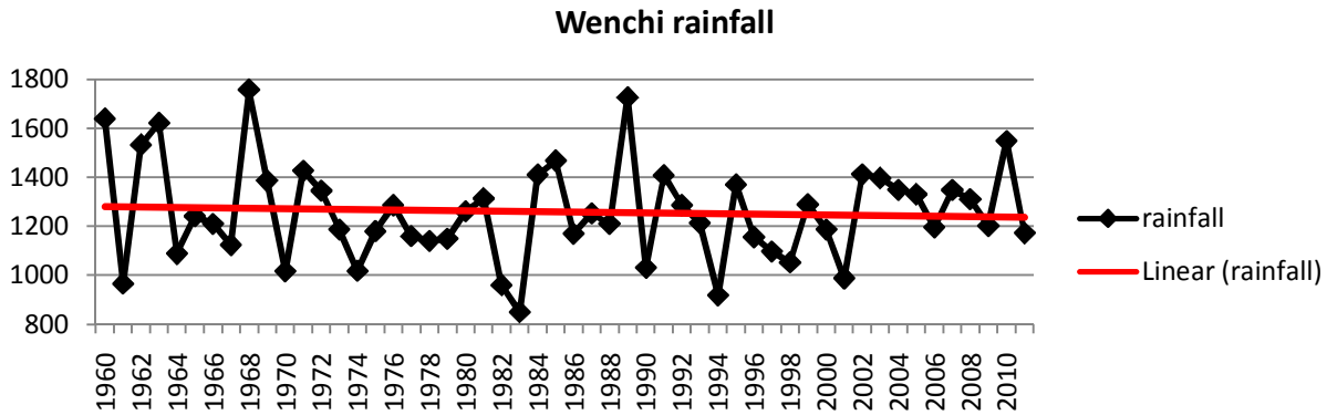
Figure 3. Annual rainfall for the Wenchi station in agro-ecological zone C.
