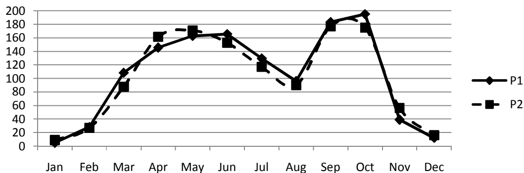
Figure 4. Rainfall for the Wenchi station showing two climatic periods: P1 (1960-1989) and P2 (1990-2011).
