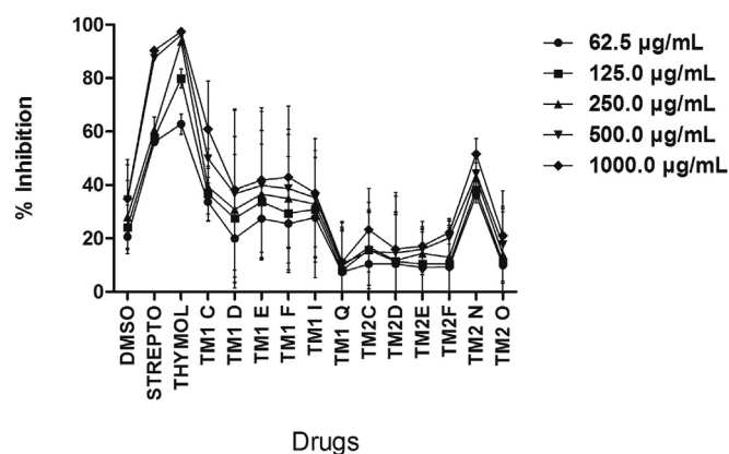
Figure 7. Effect of increasing concentrations (62.5–1000 µg/ml) of drugs on growth of E. coli . Each point is the mean % inhibition of growth \pm SD, n = 3. TM1C - 2-Isopropyl-5-methylphenyl 2-methylpropanoate, TM1D - 2-Isopropyl-5-methylphenyl butanoate, TM1E - 2-Isopropyl-5-methylphenyl-2-methyl butanoate, TM1F - 2-Isopropyl-5-methylphenyl pentanoate, TM1I - 2-Isopropyl-5-methylphenyl 2-phenylethanoate, TM1Q - 2-Isopropyl-5-methylphenyl 3-chlorobenzoate; TM2C - 2-Isopropyl-5-methylphenoxy propane, TM2D - 2-Isopropyl-5-methylphenoxy methylethane, TM2E - 2-Isopropyl-5-methylphenoxy 1-methylpropane, TM2F - 2-Isopropyl-5-methylphenoxy butane, TM2N - 2-Isopropyl-5-methylphenoxy methylbenzene, TM2O - 2-Isopropyl-5-methylphenoxy 3-chloromethylbenzene.
